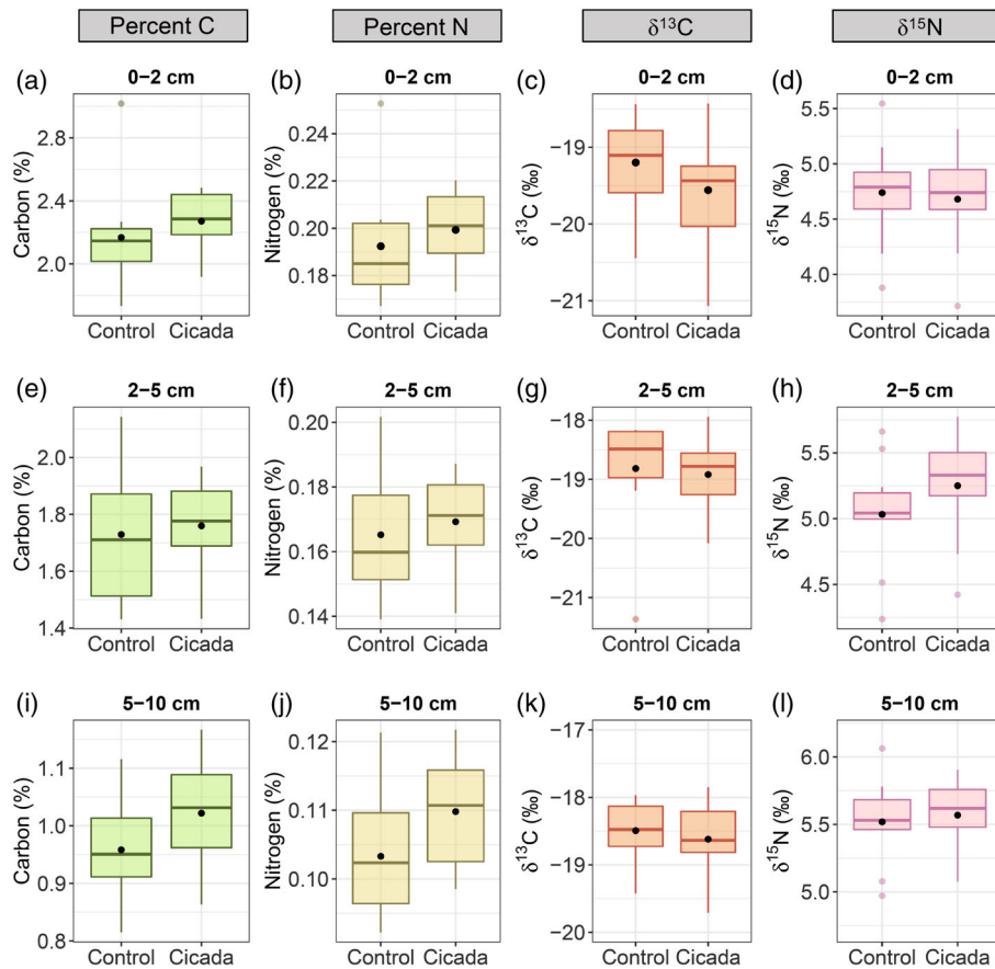
FIGURE 2 Soil C, N, \delta^{13}\text{C} , and \delta^{15}\text{N} at three soil depths (0–2, 2–5, and 5–10 cm) in the control and the cicada plots on day 100 in October 2016. A clear trend of increasing soil C and N and decreasing \delta^{13}\text{C} , though not statistically significant, can be seen throughout the three soil depths. Box plots show medians (horizontal lines inside the boxes), means (black dots), first and third quartiles (lower and upper edges of the boxes), 1.5× interquartile ranges (lines extending from the boxes), and outliers (colored dots). Note the different scales on the y-axes.
