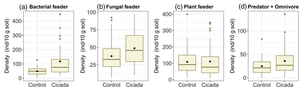
FIGURE 4 The influence of cicada carcasses on the numbers (individuals per 10 g dry soil) of different nematode feeding groups. Cicada addition significantly increased the abundance of (a) bacterial-feeding nematodes ( p < 0.001 ) and (b) fungal-feeding nematodes ( p = 0.0206 ), while it had no effect on the abundance of (c) plant-feeding nematodes ( p = 0.6728 ) and (d) predatory and omnivorous nematodes ( p = 0.4384 ) in mixed-effect models. Data from the two soil depths and seasons are pooled. Box plots show medians (horizontal lines inside the boxes), means (black dots inside the boxes), first and third quartiles (lower and upper edges of the boxes), 1.5\times interquartile ranges (lines extending from the boxes), and outliers (dots outside the boxes). Note the different scales on the y axes.
