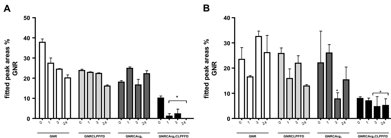
Figure 3 Percentage fitted peak area GNR and GNR-peptide with liposome over time (0–24 h). (A) 3–5 nm peak and (B) 50 nm peak. Values represent mean ± SEM of three separate experiments (* p < 0.05 ).
