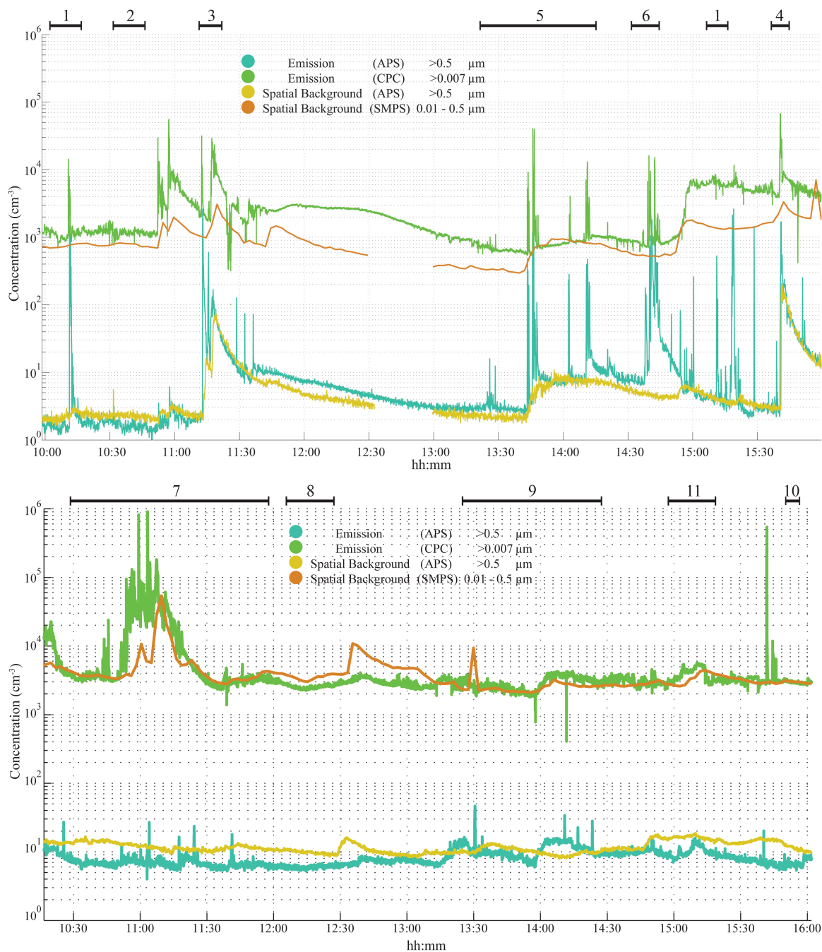
Figure 2 (a) Time series from online instruments measured in the production and sieving laboratories on the first day. Nos. 1–6 refer to Work Tasks: 1. Cleaning of deposits, 2. Harvesting, 3. Opening of the reactor, 4. Cleaning of the reactor, 5. Sieving, 6. Lathe machining. The numbers also refer to the locations in Table 1 and Fig. 1. (b) Time series from online (DRI) instruments measured in the purification laboratory on the second day. Nos. 7–11 refer to Work Tasks: 7. Purification Part I, 8. Purification Part II, 9. Functionalization Part I, 10. Functionalization Part II, 11. Grinding. The numbers also refer to the locations in Fig. 1.
