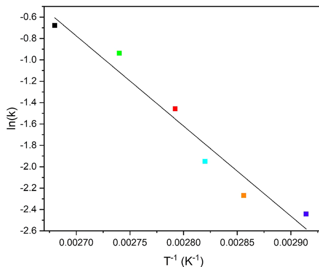
Figure 6. Arrhenius plot of \ln(k) vs T^{-1} to attain an activation energy of 70.1 \text{ kJ mol}^{-1} for the rearrangement from IPC-1P to IPC-2P.
