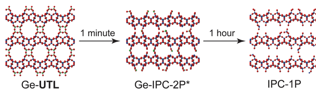
Scheme 3. Hydrolysis of Ge-UTL over the Course of 1 h a
