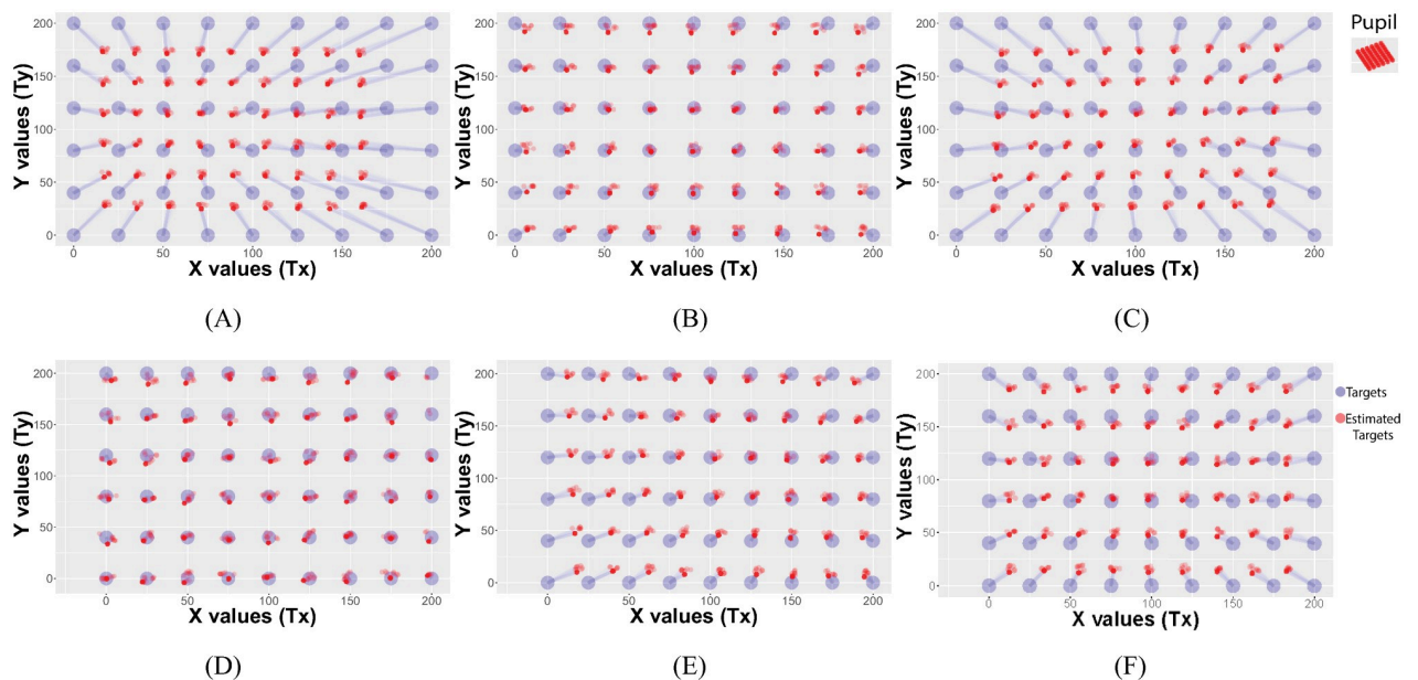
Fig 5. Reprojection of the validation points (9×6 lattice points) using the models obtained from the symbolic regression algorithm on the 6 calibration patterns. The circular and spiral calibration patterns (a. and c.) resulted in lower accuracy compared to the 9-point and rectangular calibration patterns (b. and d.).
