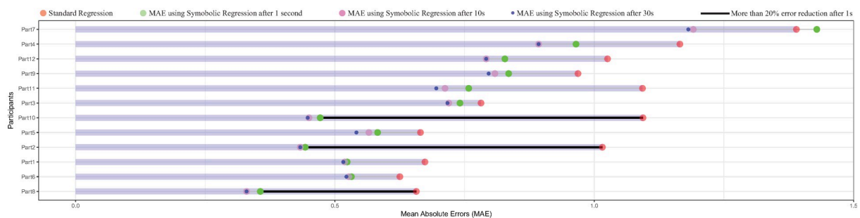
Fig 9. Reduction of the mean absolute error (MAE) in time for all participant on x-axis. A similar effect is observed for y-axis. The MAE obtained using the standard regression (orange circles) decreased significantly when using symbolic regression. It is clearly visible that the MAE obtained after 1 second (green circles) can help reducing gaze estimation accuracy in real time scenarios. For some participants, the difference between symbolic and standard regression errors (represented in bold black line) exceeded 50% (participants 10, 2 and 8). Also, note that for participant 7, the algorithm did not find directly a better model after 1 second, but a few moments later.
