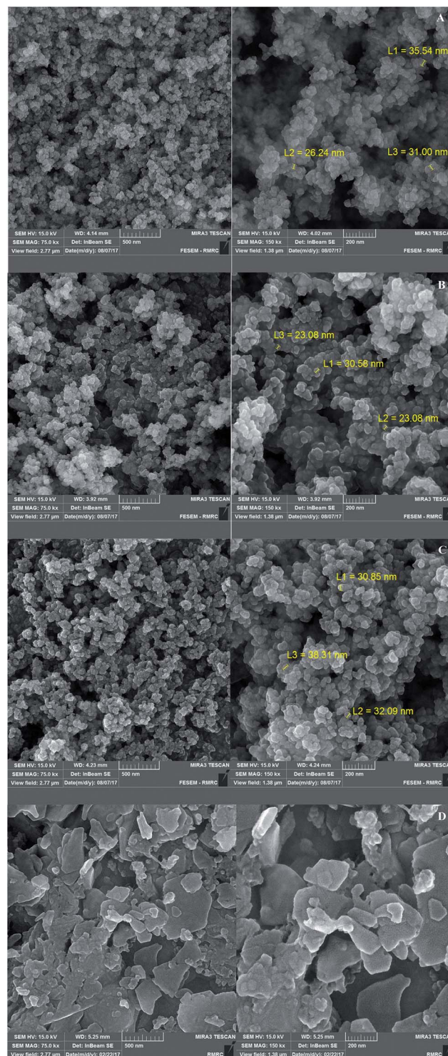
Fig. 2 FESEM images of \text{Fe}_3\text{O}_4@(\text{SiO}_2) (A), \text{Fe}_3\text{O}_4@(\text{SiO}_2@(\text{CH}_2)_3\text{Cl}) (B), \text{Fe}_3\text{O}_4@(\text{SiO}_2@(\text{CH}_2)_{35}\text{-phenyl-1H-tetrazole}) (C) and [\text{FSTet-SO}_3\text{H}]\text{Cl} (D).
