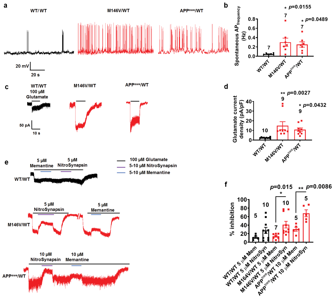
Fig. 1. AD neurons manifest increased spontaneous action potentials and glutamate-evoked currents compared to WT neurons.
