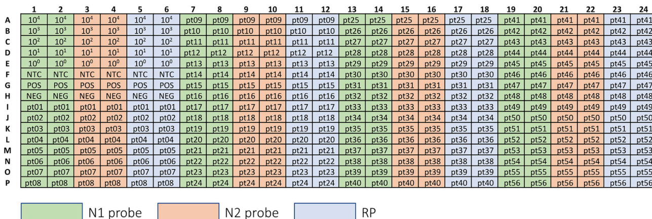
Figure 1. Sample Plate Layout for a Fully Loaded 384-Well qRT-PCR Plate Using Two- and One-Step Singleplex Assays
