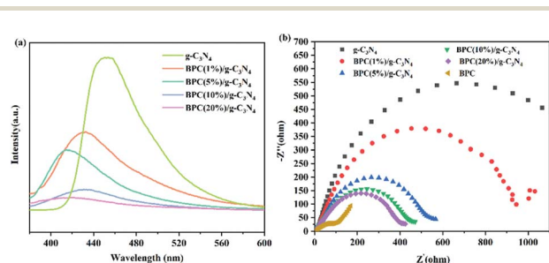
Fig. 8 Photoluminance spectra (a) and Electrochemical Impedance Spectroscopy plots (b) of the g\text{-C}_3\text{N}_4 and BPC( X\% )/ g\text{-C}_3\text{N}_4 .
