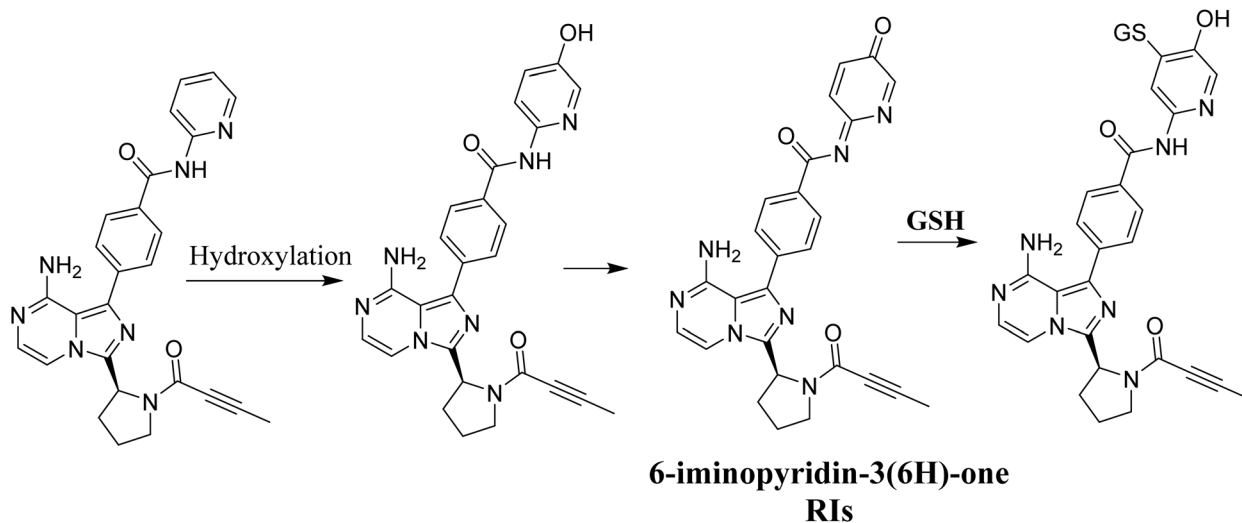
Fig. 14 Proposed bioactivation pathway of ACB to 6-aminopyridin-3(6H)-one RIs captured by GSH.
