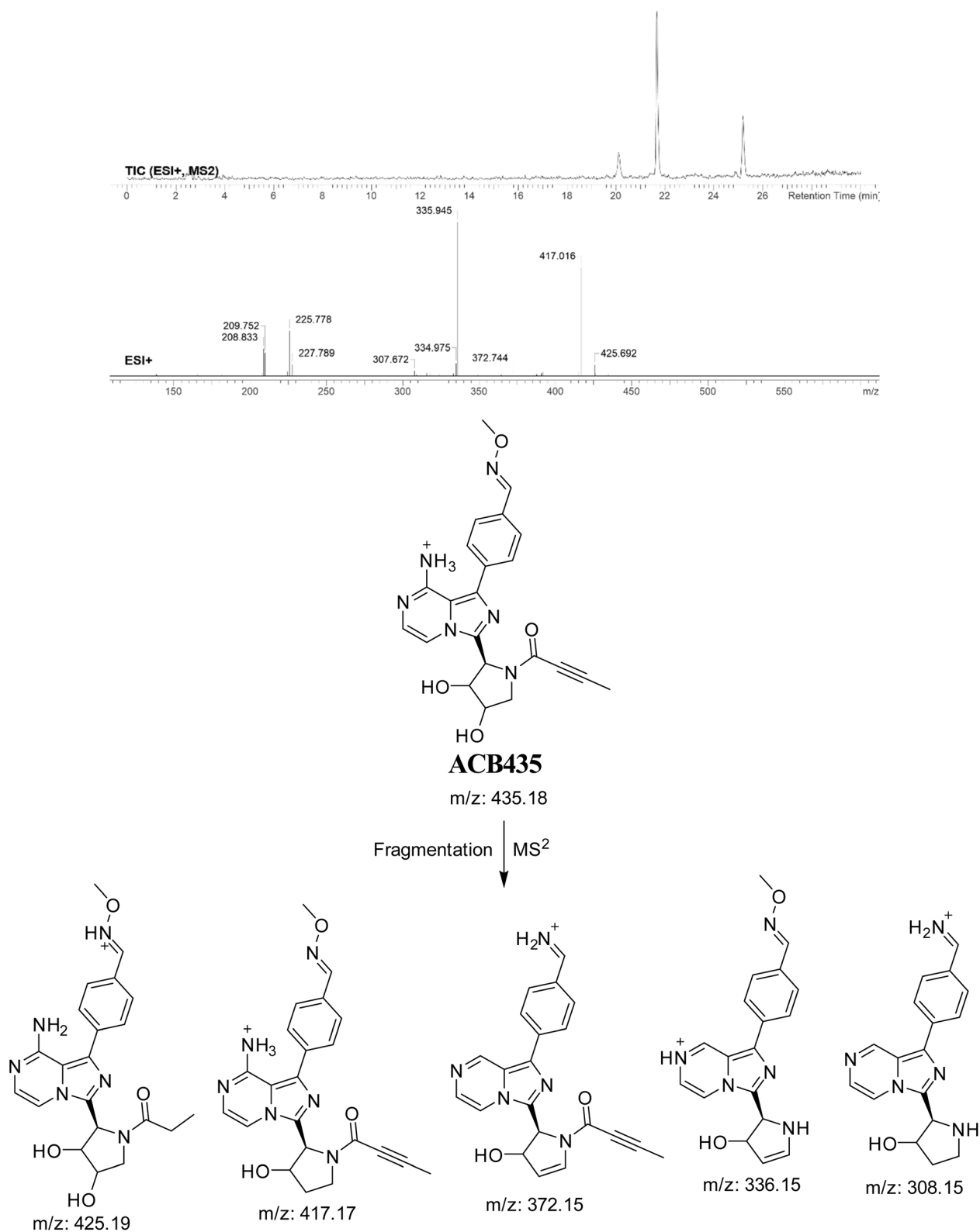
Fig. 20 PI mass spectrum of ACB435 oxime and the proposed interpretation of fragmentation of ACB435.
