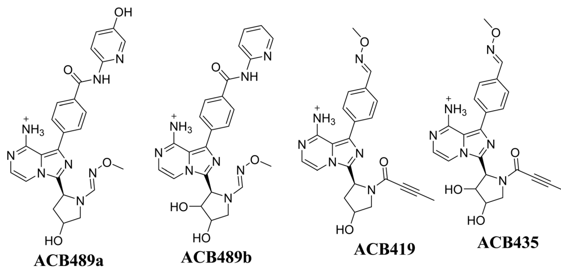
Fig. 22 Summary of proposed methoxylamine oximes of ACB.
