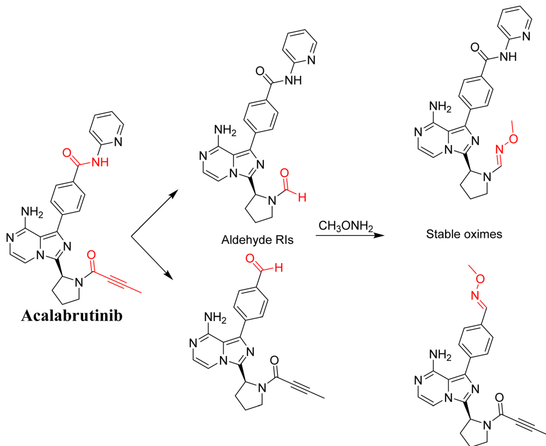
Fig. 21 Predicted bioactivation pathways of ACB to aldehyde RIs captured by methoxylamine.
