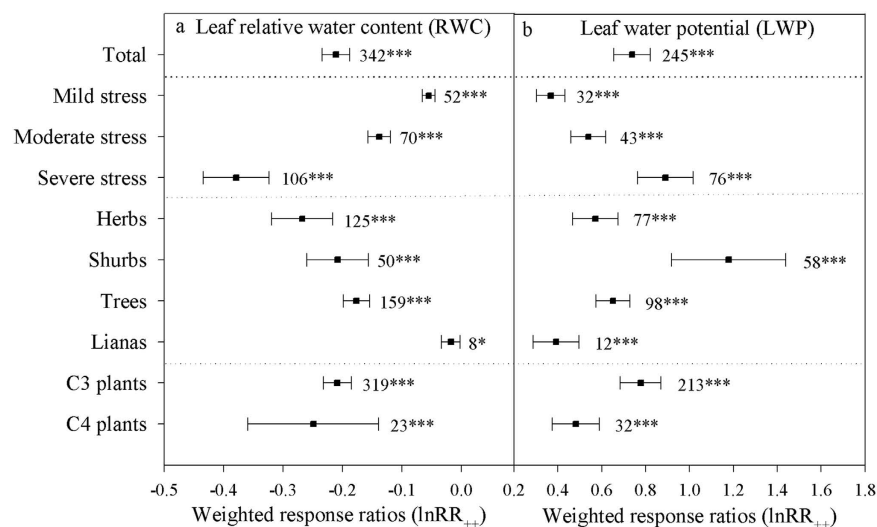
Figure 3. Weighted response ratios ( \ln RR_{++} ) of the relative water content (RWC) and leaf water potential (LWP) under different drought intensities (mild, moderate and severe) for different CO_2 -assimilation metabolic pathways ( C_3 and C_4 plants) and in different growth forms (herbs, shrubs, trees and lianas). The numbers above the symbols specify the number of data points. The error bars indicate 95% CI. Symbols (*, **, ***) after the number indicate statistical significance ( P < 0.05 , P < 0.01 , P < 0.001 , respectively).
