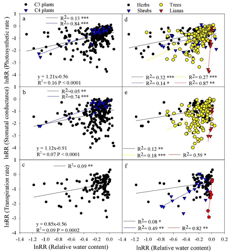
Figure 5. The relationship between the response ratios (lnRR) of the leaf relative water content (RWC) and gas exchange in all plants. The regression equation represents the correlation across all studies, and the black and blue lines represent the correlations of the C 3 and C 4 plants (panel a–c), respectively; the black, blue, yellow and red lines represent the correlations of the herbs, shrubs, trees and lianas (panels d–f), respectively.
