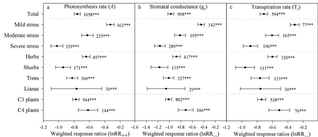
Figure 1. Weighted response ratios ( \ln RR_{++} ) of the plant photosynthesis rate ( A , panel a), stomatal conductance ( g_s , panel b) and transpiration rate ( T_r , panel c) under different drought intensities (mild, moderate and severe) for different \text{CO}_2 -assimilation metabolic pathways ( \text{C}_3 and \text{C}_4 plants) and in different growth forms (herbs, shrubs, trees and lianas). The numbers above the symbols specify the number of data points. The error bars indicate 95% CI. Symbols (***) after the number indicate statistical significance ( P < 0.001 ).
