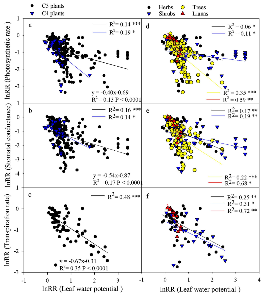
Figure 6. The relationship between the response ratios (lnRR) of the leaf water potential (LWP) and gas exchange in all plants. The regression equation represents the correlation across all studies, and the black and blue lines represent the correlation of the C 3 and C 4 plants (panels a–c), respectively; the black, blue, yellow and red lines represent the correlations of the herbs, shrubs, trees and lianas (panels d–f), respectively.
