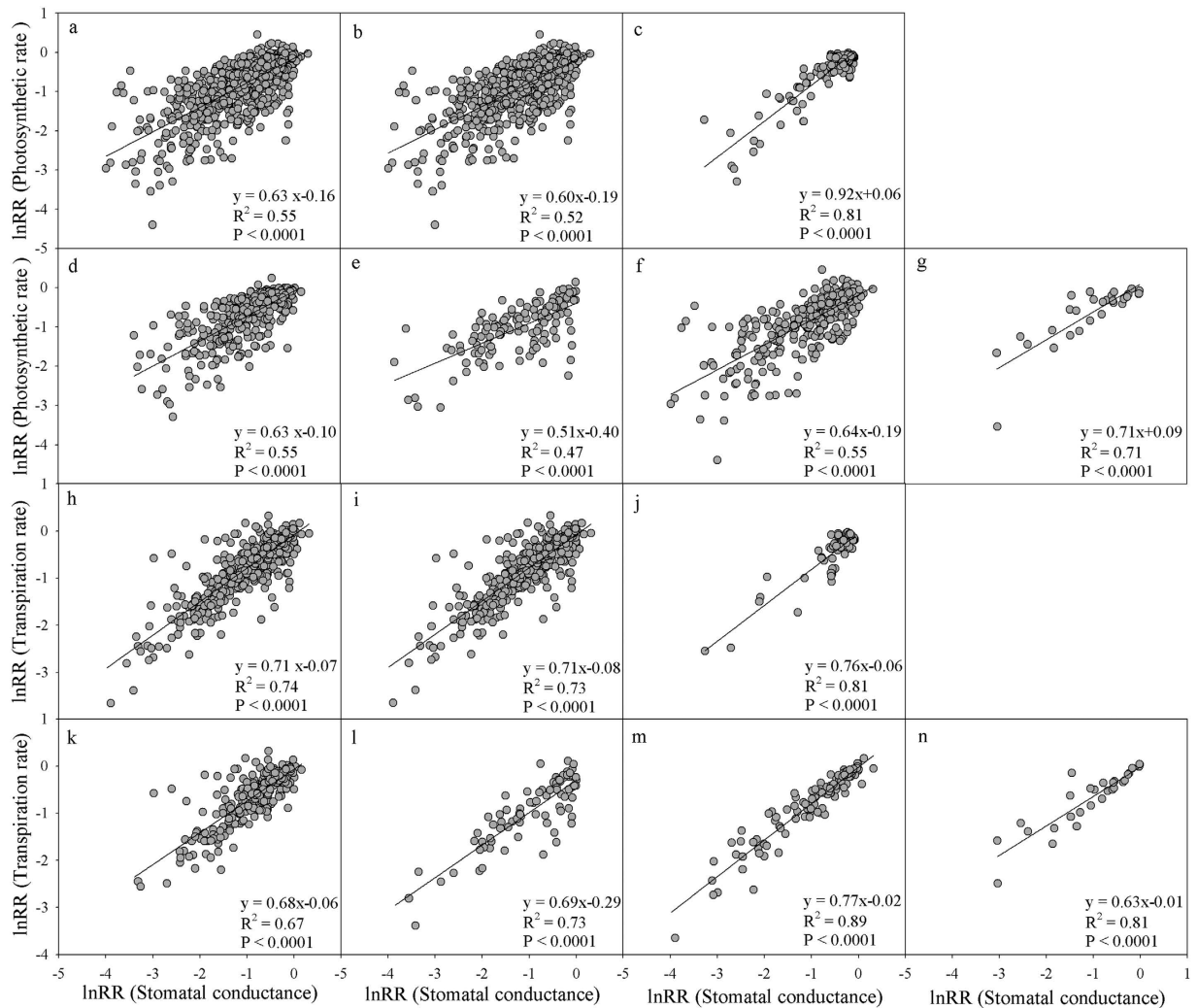
Figure 4. The relationships between the response ratios (lnRR) of the stomatal conductance ( g_s ) with the photosynthesis rate (A) and transpiration rate ( T_r ) in all plants (panels a,h), C_3 plants (panel b,i), C_4 plants (panel c,j), herbs (panels d,k), shrubs (panels e,l), trees (panels f,m) and lianas (panels g,n).
