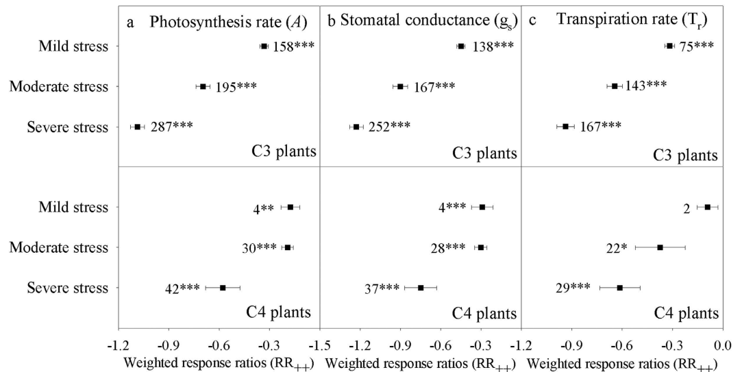
Figure 2. Weighted response ratios ( \ln RR_{++} ) of the plant photosynthesis rate ( A , panel a), stomatal conductance ( g_s , panel b) and transpiration rate ( T_r , panel c) under different drought intensities (mild, moderate and severe) for different CO_2 -assimilation metabolic pathway ( C_3 and C_4 plants). The numbers above the symbols specify the number of data points, and the error bars indicate 95% CI. The symbols (*, **, ***) after the number indicate statistical significance ( P < 0.05 , P < 0.01 , P < 0.001 , respectively).
