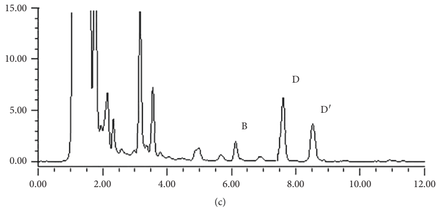
FIGURE 2: UPLC-ELSD chromatograms of standard mixture (a), CMD extract (b), and ZMD extract (c).
