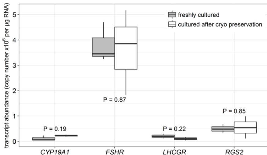
Figure 2: Comparison of cells cultured directly after isolation and after cryopreservation. The cells were cultured at a density of 1 \times 10^5 cells per well. The gene expression of several marker transcripts was evaluated and revealed no difference between cultured cells with or without an initial cryopreservation. The boxplot shows the median of n = 3 . Two-tailed Student's t -test, the p -values are included. This figure is reproduced from Baufeld and Vanselow 16 . Please click here to view a larger version of this figure.
