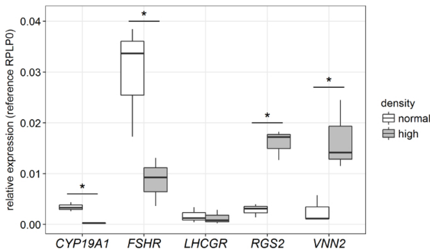
Figure 4: Abundance of functional key transcripts in granulosa cells cultured at a normal vs. a high plating density. Bovine GC cultured under serum-free conditions for 8 d revealed a specific regulation of several selected marker genes. The boxplot displays the median of n = 3 individual replicates. p < 0.05 , two-tailed Student's t -test. Please click here to view a larger version of this figure.
