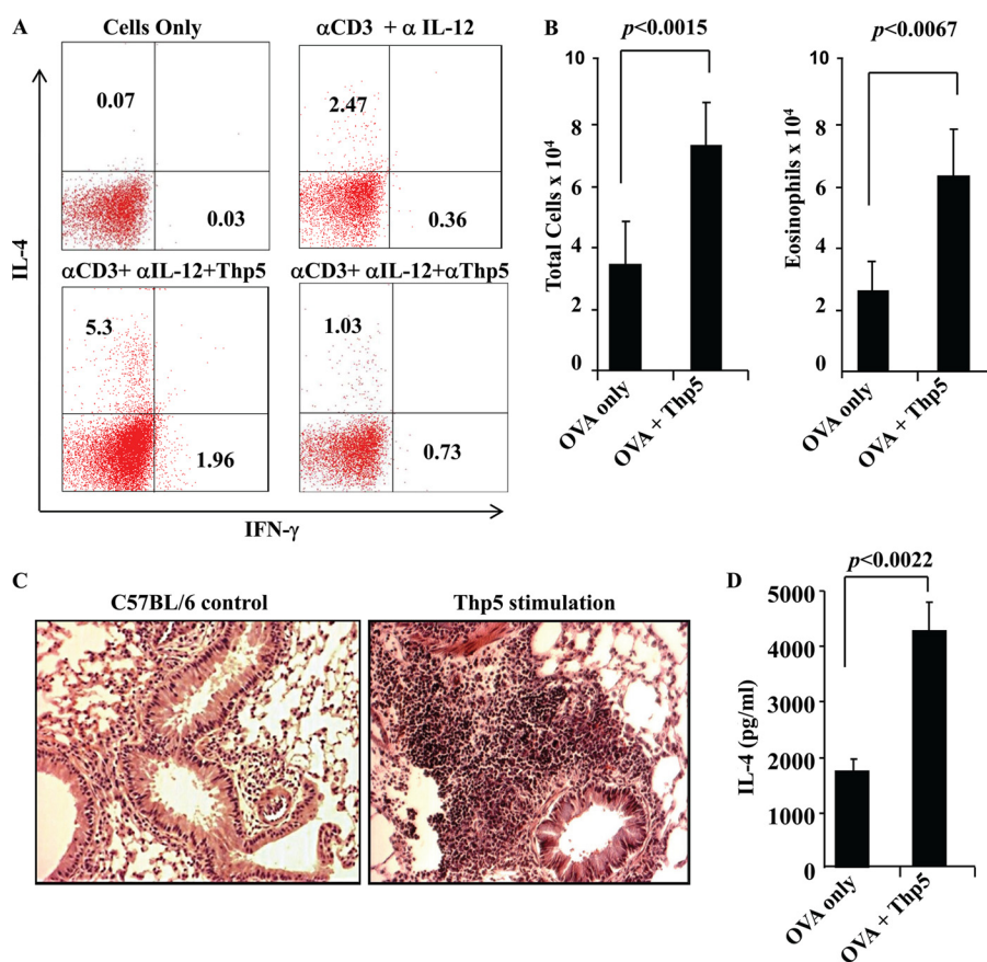
FIGURE 3. Thp5 induces Th2 cell differentiation and AAI. A, Th2 cell differentiation by Thp5 determined by intracellular IL-4 production in the presence of anti-IL12. B, inflammatory cells in the BAL fluid of mice with ovalbumin (OVA)-induced AAI. C, histological analysis of lungs of wild-type littermates (C57BL/6) induced for AAI and treated with or without Thp5. D, Th2 cytokines in the BAL fluid of mice induced for AAI and treated with Thp5. Results shown here are representative of three independent experiments.
