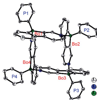
Fig. 5 Molecular structure of [ 10a ] 4 . H atoms, isopropyl groups, and C 6 D 6 solvent molecules are omitted for clarity. 'Bo' and 'P' denote the planes of the phenylpyridyl-fused borole and the Tip phenyl groups, respectively. Selected bond lengths (Å) and angles (°): B Bo1 –N Bo4 1.655(2), B Bo2 –N Bo1 1.652(2), B Bo3 –N Bo2 1.644(2), B Bo4 –N Bo3 1.644(2), B Bo1 –B Bo2 5.420(2), B Bo2 –B Bo3 5.365(2), B Bo3 –B Bo4 5.407(2), B Bo4 –B Bo1 5.402(2), ∠Bo1–Bo2 89.70(2), ∠Bo2–Bo3 81.78(2), ∠Bo3–Bo4 89.22(2), ∠Bo4–Bo1 78.44(2), ∠Bo1–Bo3 33.29(3), ∠Bo2–Bo4 33.21(2).
