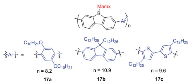
Scheme 20 9-Mamx-9-borafluorene-based polymers.
