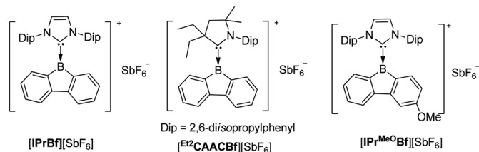
Scheme 24 Carbene-stabilized borafluorenum cations.
