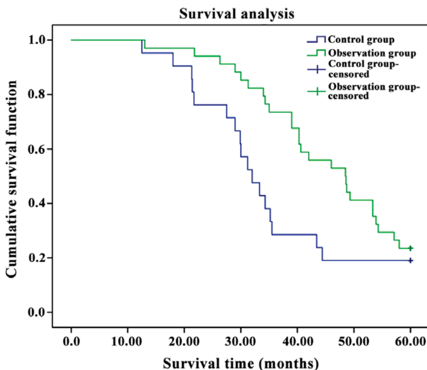
Figure 1. Survival curve of patients; the survival analysis of Kaplan-Meier at P&lt;0.05.
