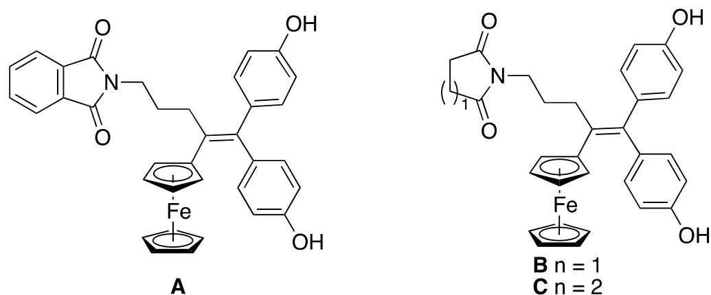
Figure 1. Recently reported imido-ferrocenyl diphenols A–C with high anticancer activity.
