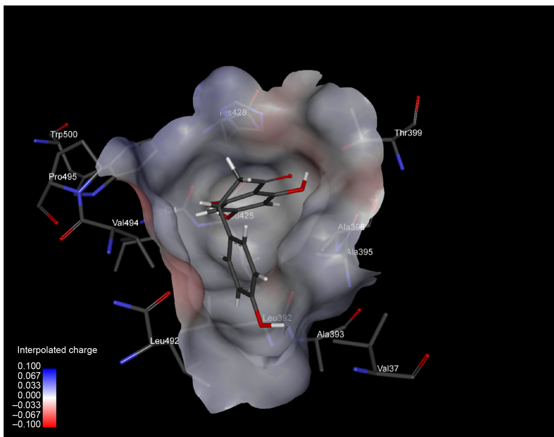
Figure 2 An inside view of binding pocket of HCV-NS5B, with a small drug molecule (naringenin) firmly bound. Note: Interpolated charge (color intensity from blue to red) of binding pocket residues (in sticks) is represented. Abbreviations: HCV, hepatitis C virus; NS5B, nonstructural protein 5B.
