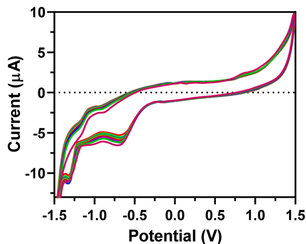
Fig. 2 The electrodeposition process of BFO NPs on the surface of the EEGO-AG-modified GCE ( N = 10 cycles, scan rate 100 \text{ mV s}^{-1} , PBS 50 mM, pH 7.0).
