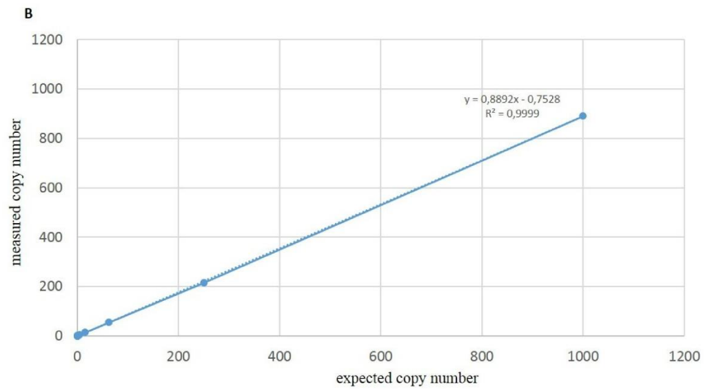
Figure 4. Linear correlation between values of measured copy number quantified by ddPCR ( y -axis) and the known copy number composition of samples obtained by the mixture of gDNAs from A.1 and B.1 monoconidial isolates ( x -axis). (A) Quantification of allele A143 in samples of group 1. (B) Quantification of allele G143 in DNA mixture of group 2.
