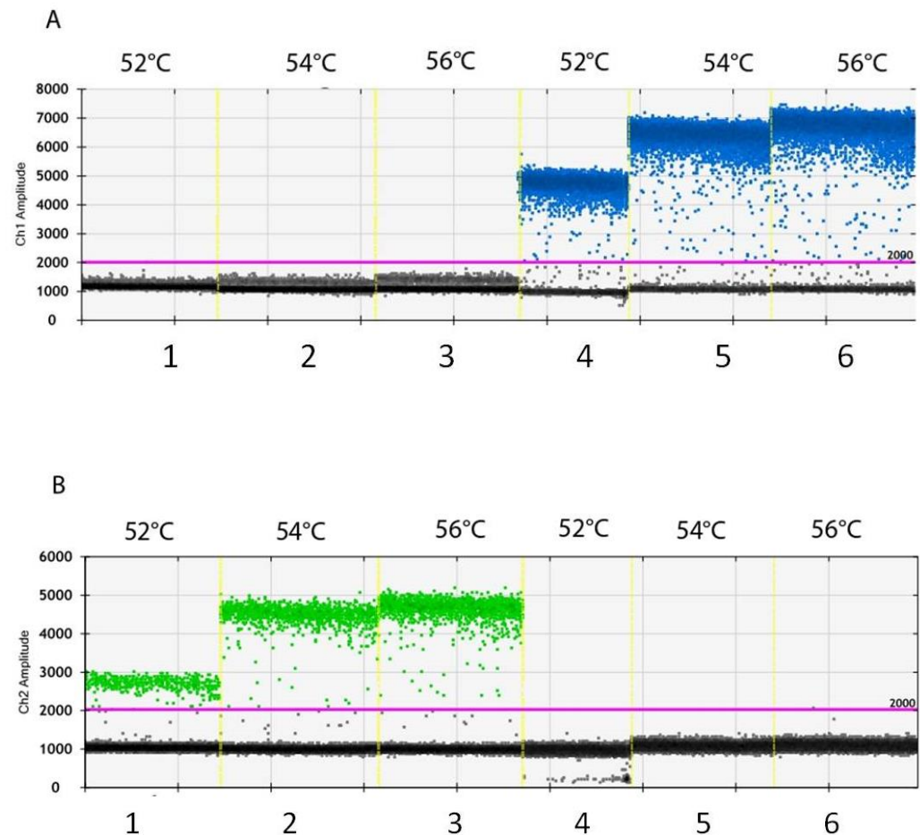
Figure 2. Amplitudes from channel 1 (FAM) (A) from channel 2 (HEX) (B) obtained during the second experiment to optimize the annealing/extension step and select the most performant DNA quantity. ddPCR assay was conducted for annealing/extension step, run at 52 °C (lanes 1, 4), 54 °C (lanes 2, 5), or 56 °C (lanes 3, 6) adding to the reaction 0.1 ng of gDNA purified from the monoconidial isolate B.1 (lanes 1–3) or from monoconidial isolate A.1 (lanes 4–6).
