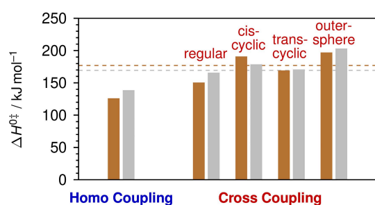
Figure 5. Reaction barriers for the homo- and cross-coupling pathways of [\text{RCuMe}_3]^- and [\text{RAgMe}_3]^- (copper- and silver-colored, respectively; \text{R}=\eta^1 -allyl) obtained from DLPNO-CCSD(T)//PBE-D3BJ calculations. The dashed lines indicate the DLPNO-CCSD(T)//PBE-D3BJ threshold energies for the homolytic cleavage of the M–R bond of the complexes, which is the energetically most favorable dissociation reaction according to the coupled-cluster calculations.
