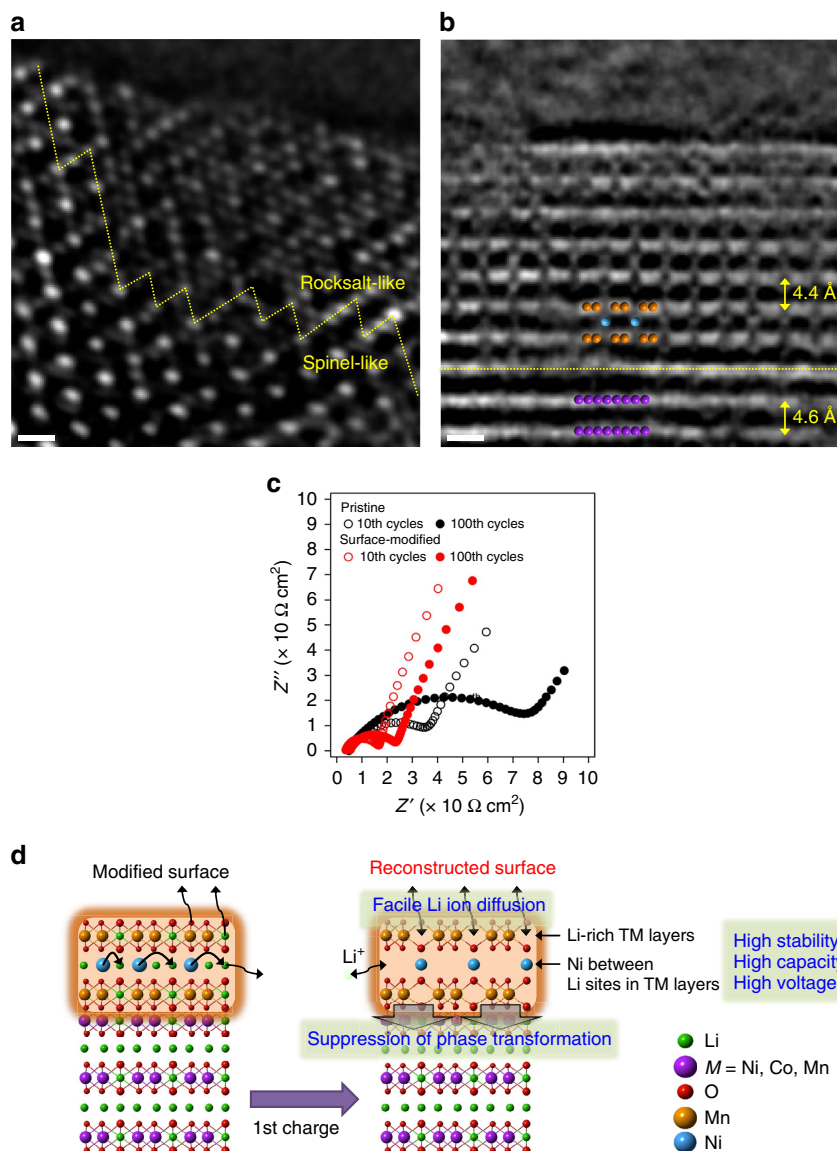
Figure 4 | Effect of atomic-level surface modification. (a,b) HAADF-STEM images of (a) the pristine electrode and (b) the surface-modified electrode with 5 wt% Li 2 MnO 3 after the first charge. a,b were obtained along the rhombohedral [100] (= cubic spinel [110]) and monoclinic [100] directions, respectively. (c) Nyquist plots of both electrodes after the tenth and hundredth cycles. (d) Graphical illustration of the effect of the surface modification. The green, purple, red, orange and blue circles represent Li, TM ( M = \text{Ni, Co and Mn} ), O, Mn and Ni, respectively. Scale bars, 5 Å.
