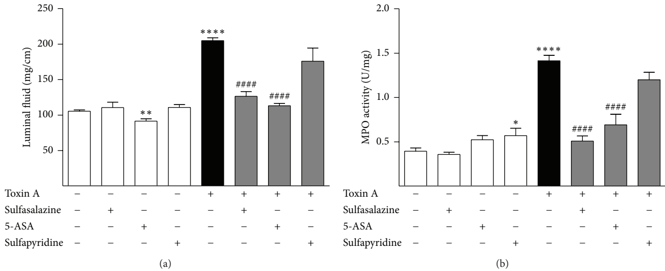
FIGURE 3: Effects of sulfasalazine, 5-ASA, and sulfapyridine on toxin A-induced colonic luminal fluid accumulation and MPO activity. Sulfasalazine was administered in the drinking water at a dose of 100 mg/kg-day for 5 days. 5-ASA and sulfapyridine were administered as pretreatments for 30 minutes before toxin A was injected into isolated colonic segments. (a) Toxin A stimulation of colonic luminal fluid accumulation and the inhibition of this effect by chronic treatment with sulfasalazine or acute treatment with 5-ASA or sulfapyridine. (b) Toxin A stimulation of colonic MPO activity and the inhibition of this effect by chronic treatment with sulfasalazine or acute treatment with 5-ASA or sulfapyridine. * P < 0.05 versus no treatment; ** P < 0.01 versus no treatment; **** P < 0.001 versus no treatment; #### P < 0.0001 versus toxin A.
