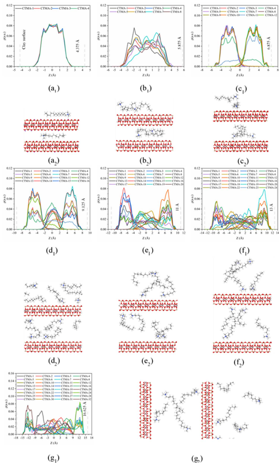
Fig. 8 Density distributions ( \rho(z) ) along z direction and snapshots ( \rho(z) ) from MD simulations of CTMA + -Mt: (a) 0.33CEC; (b) 0.66CEC; (c) 1.00CEC; (d) 1.33CEC; (e) 1.66CEC; (f) 2.00CEC; (g) 2.66CEC. Blue spheres = N; grey spheres = C; white spheres = H; red spheres = O. The vertical gray dotted line shows the position of the Os atoms. To clearly show the CTMA + arrangement, only part of the CTMA + cations are selected in the snapshot.
