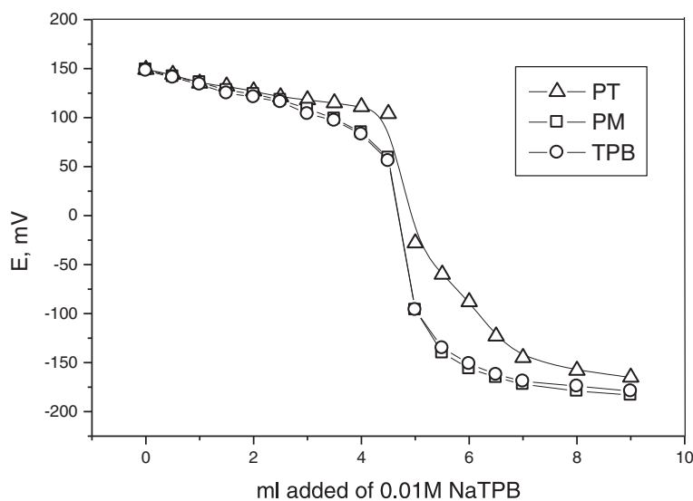
Figure 4 Typical potentiometric titration curves of 5.0 ml of 1 \times 10^{-2} M MOX with 1 \times 10^{-2} M sodium tetraphenylborate using moxifloxacin membrane sensors.
