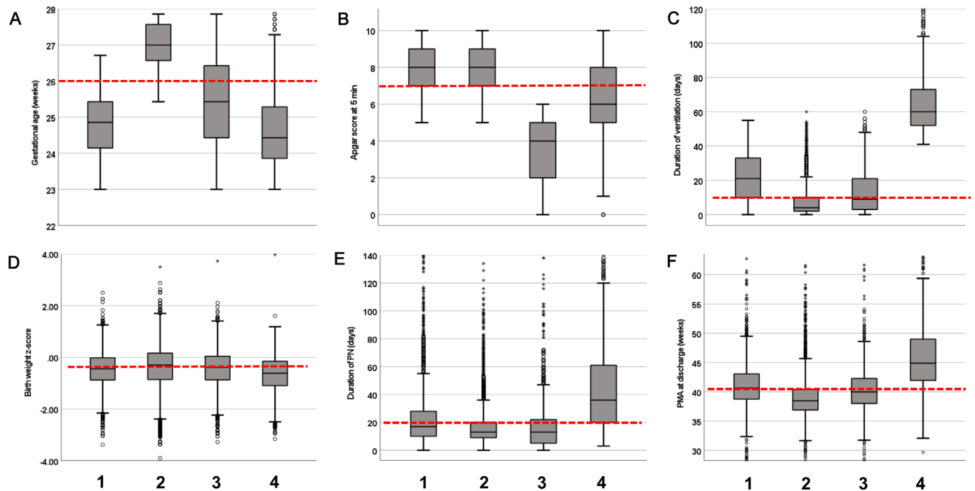
Figure 4 Boxplots of the gestational age (A), Apgar score at 5 min (B), duration of ventilation (C), birth weight z-score (D), duration of parenteral nutrition (PN) (E) and postmenstrual age (PMA) at discharge (F) in the four clusters. The median value for each parameter for the whole population is depicted as a dashed line. The whiskers represent the maximum and minimum values. The asterisks are extremes (at least three box lengths from the median) and the circles are outliers (1.5 box lengths from the median).
