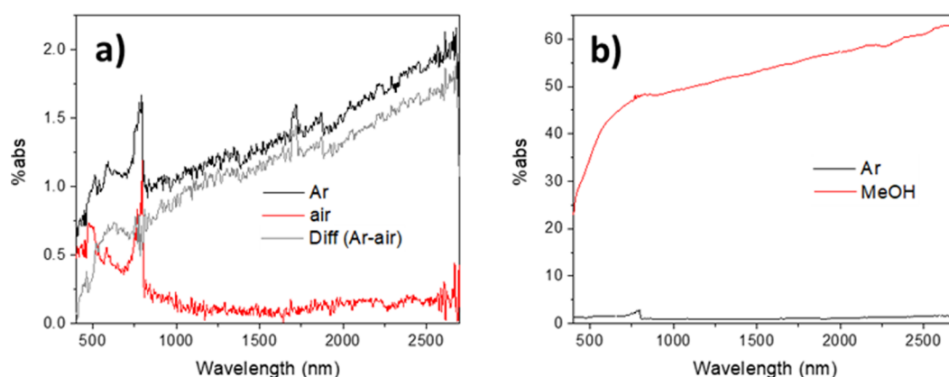
Figure 2. Photoinduced absorption spectra (PIA) of anatase \text{TiO}_2 powder under 365 nm excitation in the presence of (a) air and (b) methanol vapor in argon. A reference spectrum acquired under 100% argon is also shown in each panel for comparison. In (a), the difference spectrum between the two spectra collected under different atmospheres is also shown in gray. The discontinuity at 800 nm is an artifact occurring at the detector and grating changeover wavelength. The average excitation intensity is estimated to be around 1 \text{ mW}/\text{cm}^2 . Apart from the MeOH trace in (b), all other traces are the average of several repeats on the same sample (three repeats for the data shown in (a) and five repeats for the argon trace in (b)). Data for individual repeats can be found in Figures S6 and S7 in section V in the Supporting Information for traces in (a) and (b), respectively.
