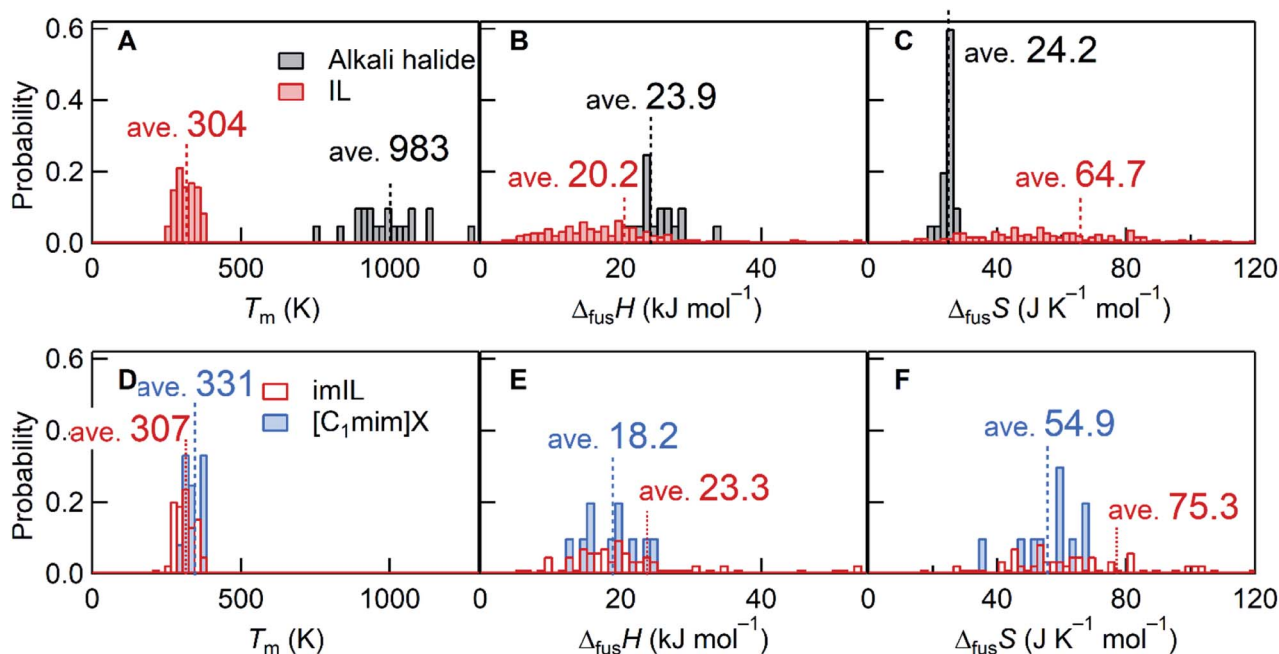
Fig. 1 Histogram comparisons of T_m , \Delta_{fus}H , and \Delta_{fus}S . (A–C) 20 alkali halides 10 versus 257 ILs 11,12 and (D–F) 84 imILs versus 12 [\text{C}_1\text{mim}]\text{X} . For [\text{C}_1\text{mim}]\text{X} , this work reported 10 data and the two additional data were taken from the ref. 41 and 42 (Table S3†). Bin widths for the T_m , \Delta_{fus}H , and \Delta_{fus}S histograms were 20 K, 1 \text{kJ mol}^{-1} , and 2 \text{J K}^{-1} \text{mol}^{-1} , respectively. For ILs and imILs, several data of \Delta_{fus}H and \Delta_{fus}S are out of range of the figures.
