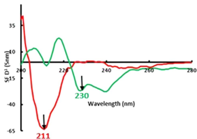
Fig. 3 Zero-crossing points on the first derivative synchronous spectra ( \Delta\lambda = 5 nm) of 200 \text{ ng mL}^{-1} VAS (green line) and 190 \text{ ng mL}^{-1} SAB (red line) in 0.1 M \text{H}_2\text{SO}_4 .
