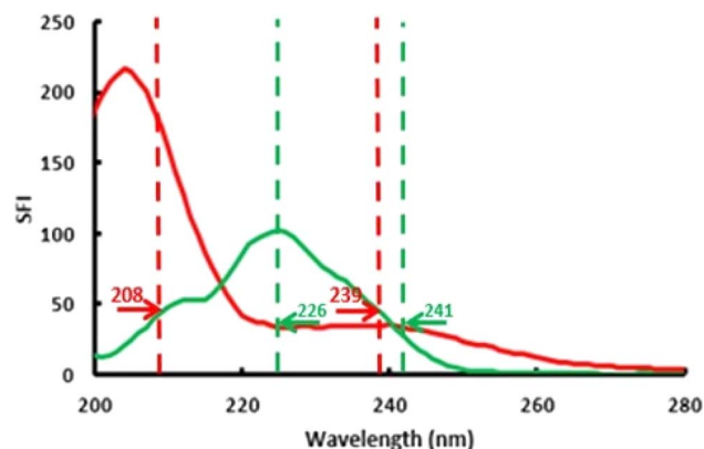
Fig. 2 Dual wavelength points on the synchronous fluorescence spectra ( \Delta\lambda = 130 nm) of 200 \text{ ng mL}^{-1} VAS (green line) and 190 \text{ ng mL}^{-1} SAB (red line) in 0.1 M \text{H}_2\text{SO}_4 .
