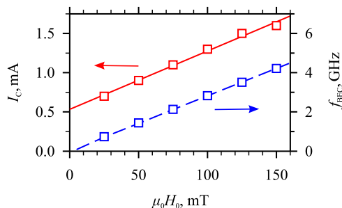
Fig. 5 Dependence on the magnetic field. Static-field dependence of the critical current I_C and of the BEC frequency f_{BEC} . A solid line is the linear fit of the experimental data. Dashed curve—calculated frequency of the lowest-energy magnon state f_{min} .
