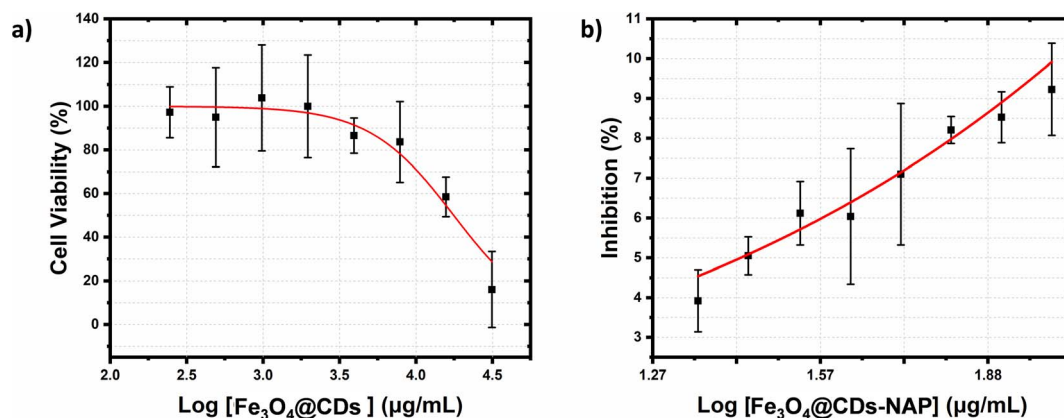
Fig. 7 HeLa cancer cell viability curves after 24 h incubation of (a) Fe 3 O 4 @CD nano hybrids and (b) inhibition of HeLa cancer cell curves after 24 h incubation of loaded Fe 3 O 4 @CDs-NAP nano hybrids. CC 50 and IC 50 values were plotted on the red fitted curves that resulted from dose-response mode on the Origin software. All data are expressed as mean \pm SD with n = 3 .
