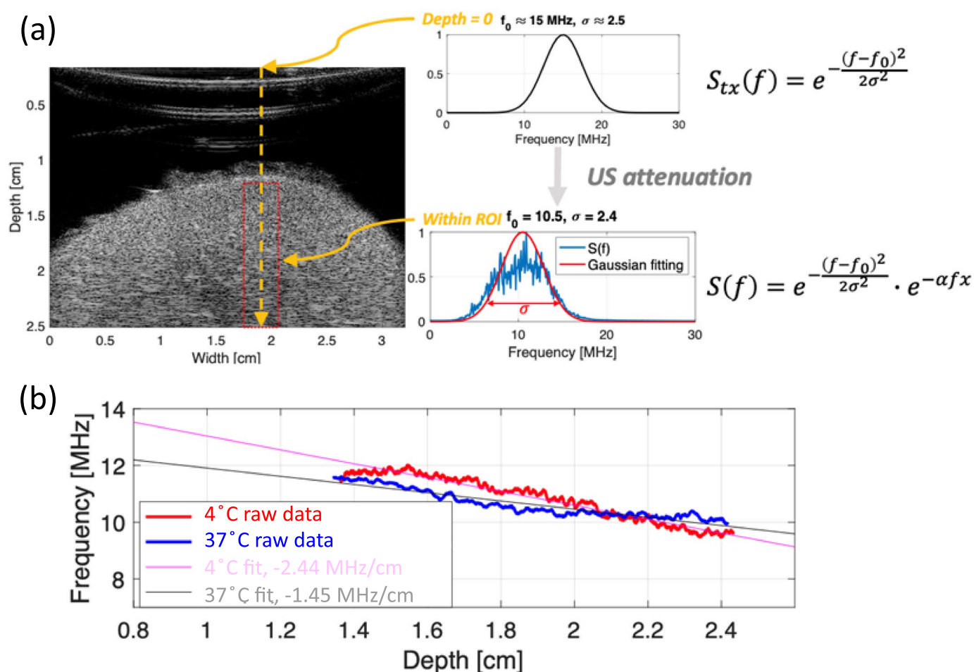
Extended Data Fig. 5 | Calculation of temperature-dependent attenuation coefficients for renal H-scan. (a) Schematic illustrating computation of temperature-dependent attenuation coefficients. (b) Peak frequency as function of depth for two temperatures relevant to the measurements of kidney
