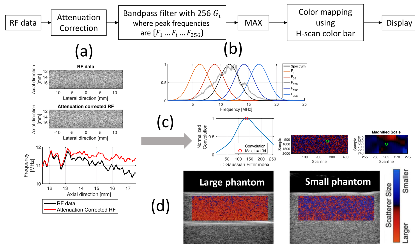
Extended Data Fig. 3 | Illustration of the H-scan algorithm. (a) Attenuation correction of the backscattered RF data is performed by dividing each ROI into 10 zones and re-incorporating the exponential decay of the backscattered power due to depth- and frequency-dependent attenuation. The dominant frequency of the backscattered signals is displayed as a function of axial depth. (b) A total of 256 Gaussian filters were then designed, each with a center frequency ranging from -70\% to +70\% of the probe center frequency of 15 MHz. (c) Each bandpass Gaussian filter was used on the frequency domain of the attenuation-corrected
