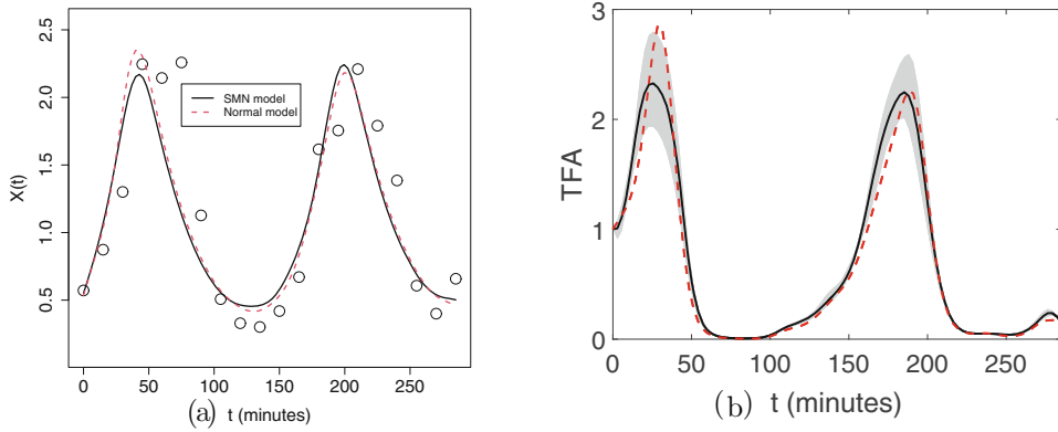
Figure 2. Example of inference applying the SMN model (solid lines) and normal model (slashed lines) with real microarray data from fission yeast. a The observations of gene expressions (circles) and the numerical solutions of the gene regulation mixed-effects ODE model (4.1) for Gene 12; b the posterior mean estimates of \eta(t) ; the shaded area denotes the 95% credible intervals of the TFA \eta(t) under the SMN model.
