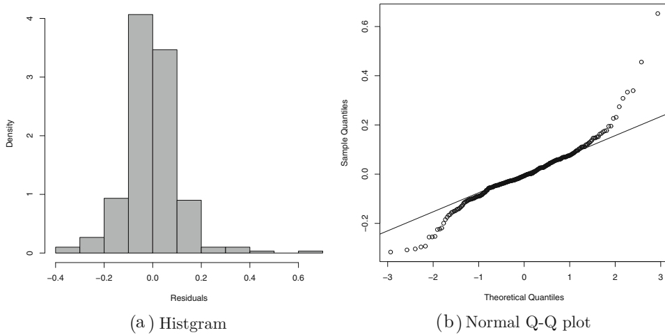
Figure 1. The histogram and the normal Q–Q plot of the obtained residuals assuming normal distributions for observations and random effects in the gene regulation ODE model (4.1) with the fission yeast cells.
