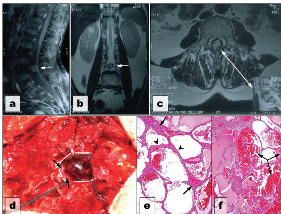
Fig. 1 a: Sagittal lumbar spine, T 1 - weighted: well-defined, high signal lesion, located into the spinal canal behind L4 vertebral body. b: Coronal lumbar spine, T 2 -weighted: well-circumscribed, mixed-signal, intradural lesion, located between cauda equina nerve roots. c: Axial lumbar spine, T 2 -weighted: welldefined, intradural, round, occupying the spinal canal almost completely. d: Intraoperative view: well circumscribed tumor located between cauda equina nerve roots ( black arrows ). e: Irregularly dilated and packed vascular spaces separated by connective tissue walls, thickened by fibrosis ( black arrowheads ) and housing in many places a visible inflammatory cell population. f: Enlarged vascular spaces by the rupture of the thin connective tissue walls, with intratumoral hemorrhage and clot tendency ( black arrows ).
