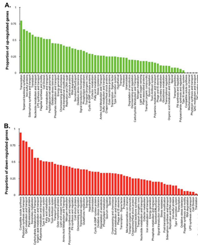
Fig 5. Proportion of up-regulated and down-regulated genes of Pseudomonas syringae B728a. Proportion of up-regulated and down-regulated genes of Pseudomonas syringae B728a in those functional gene categories that exhibited differential expression in immobilized cells as compared to planktonic cells 2 hours after application to a filter surface. (A) Proportion of up-regulated genes in each functional gene category and (B) proportion of down-regulated genes in each functional gene category.
