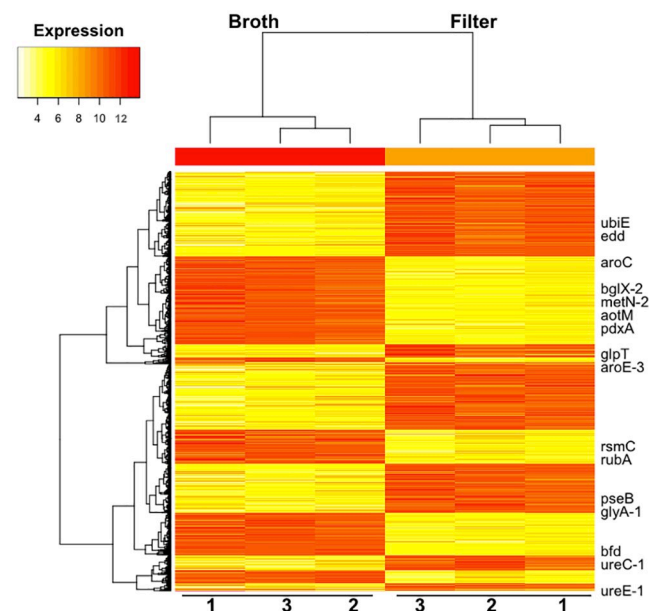
Fig 3. Heat map illustrating different patterns of gene expression in cells of Pseudomonas syringae B728a. Heat map illustrating different patterns of gene expression in cells of Pseudomonas syringae B728a 2 hours after application to a filter surface compared to that in broth culture. Red indicates high expression and yellow indicates low expression.
