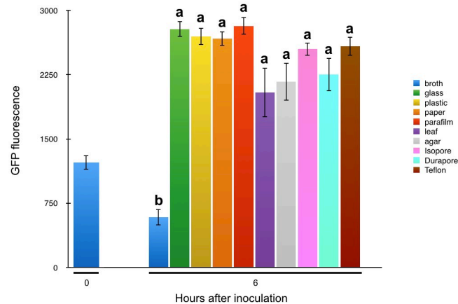
Fig 2. The expression of syfA increases rapidly after immobilization of cells of Pseudomonas syringae B728a. Gene expression is estimated as the mean GFP fluorescence of individual cells harboring a plasmid in which the syfA promoter was fused to a gfp reporter gene when harvested 6 hours after application to glass (green), polycarbonate plastic (yellow), paper (orange), parafilm (red), bean leaves (purple), agar (grey), Isopore filters (pink), Durapore filters (aqua), Teflon filters (brown), or recovered from broth cultures at the time of application to surfaces or after 6 hours (blue). The vertical bars represent the standard error of the mean GFP fluorescence for a given cell. Bars sharing a letter are not significantly different at p < 0.05 by Tukey HSD test.
