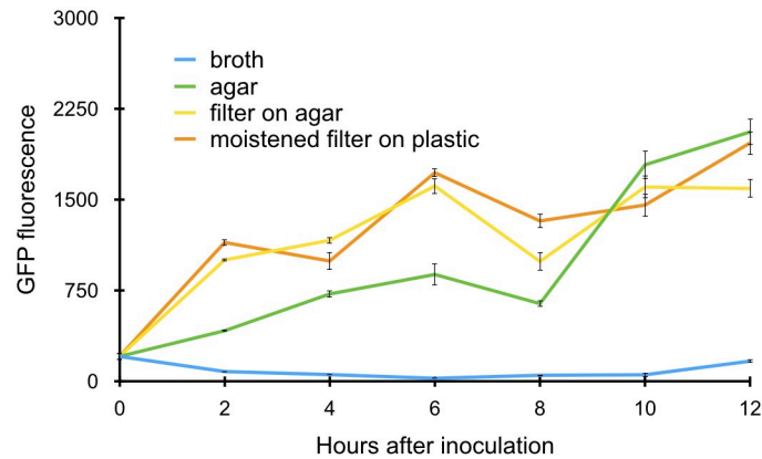
Fig 1. Induction of syfA expression in cells of Pseudomonas syringae B728a as a function of time. Gene expression is estimated as the mean GFP fluorescence of individual cells harboring a plasmid in which the syfA promoter was fused to a gfp reporter gene when harvested from these conditions at the various times shown on the abscissa. 7,038 cells were evaluated in total for control cells that remained in a broth culture (blue); 3,068 cells were evaluated after application to an agar surface (green); 10,184 cells were evaluated after application to filters placed on an agar surface (yellow); and 3,791 cells were evaluated after application to a filter moistened with KB broth that was then placed on plastic (orange). The vertical bars represent the standard error of the mean GFP fluorescence for a given cell.
