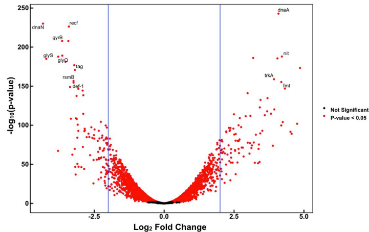
Fig 4. Volcano plot illustrating the differential expression of genes in Pseudomonas syringae B728a. Volcano plot illustrating the differential expression of genes in Pseudomonas syringae B728a 2 hours after application to a filter surface. Genes that are significantly differentially expressed compared to that in broth culture are shown in red, and those that do not differ are shown in black.
