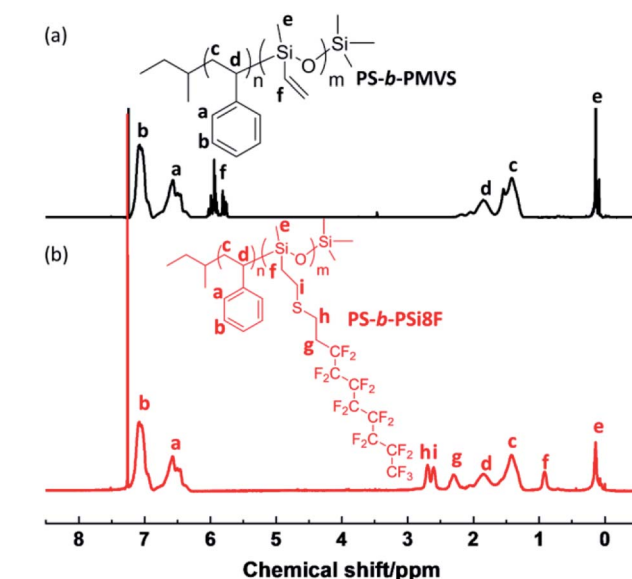
Fig. 1 Representative 1 H NMR spectra of (a) PS- b -PMVS (SV13.6) and (b) PS- b -PSi8F (SF20.8) in CDCl 3 solvent.
