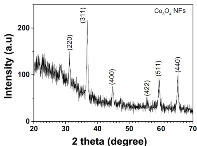
Fig. 6 XRD pattern of the annealed \text{Co}_3\text{O}_4 NFs.
