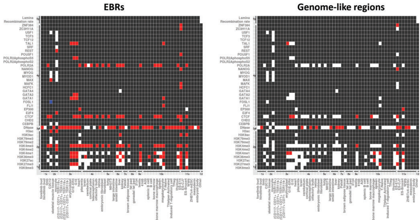
Fig. 4. —Heat maps representing significant association found when comparing Rodentia EBRs (left panel) and control genome-like regions (right panel) with epigenetic modifications in 58 different mouse cell lines based on 10,000 permutation test with randomization ( P -value < 0.05 ). Red squares indicate positive association (enrichment with P -value \leq 0.05 ); white squares indicate no statistical association ( P -value > 0.05 ), whereas blue squares indicate depletion ( P -value \leq 0.05 ). Black squares reflect no data available. The x-axis represents: (1x) Skeletal system, (2x) Muscular system, (3x) Circulatory system, (4x) Nervous system, (5x) Respiratory system, (6x) Digestive system, (7x) Excretory system, (8x) Endocrine system, (9x) Reproductive system, (10x) Lymphatic system, (11x) Stem cells, and (12x) Other. The y-axis shows: (1y) Histone modifications leading to “close” chromatin, (2y) Histone modifications associated with “open” chromatin, (3y) DNase-seq, (4y) Transcription factors, (5y) Other.
