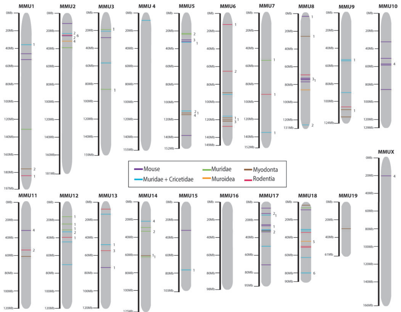
Fig. 2. —EBRs mapped in the mouse genome. The positions of EBRs detected (lineage and clade-specific) are color-coded (see inset legend) along mouse (MMU, M. musculus ) chromosomes. The number of protein-coding genes detected within each EBR is depicted on the right of each chromosome.
