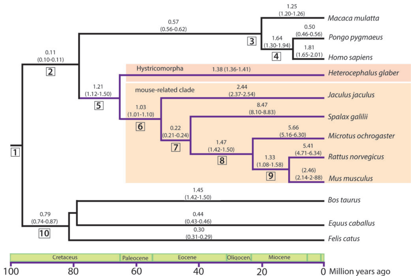
FIG. 1. —EBRs mapped in the time tree of the mammalian species included in the study. Time tree was based on divergence times (autocorrelated rates and hard-bounded constraints) described by Meredith et al. (2011), to the exception of two species ( M. musculus and R. norvegicus ) and one clade (Muridae) which were estimated from dos Reis et al. (2012) time tree. In the upper section of each branch, the mean rate of EBRs per Myr and the range (in brackets) is shown. Numbers framed in squares represent mammalian phylogenetic nodes: 1: Boreoeutheria; 2: Euarchontoglires; 3: Catarrhini; 4: Hominoidea; 5: Rodentia; 6: Myodonta; 7: Muroidea; 8: Cricetidae + Muridae; 9: Muridae; 10: Laurasiatheria.
