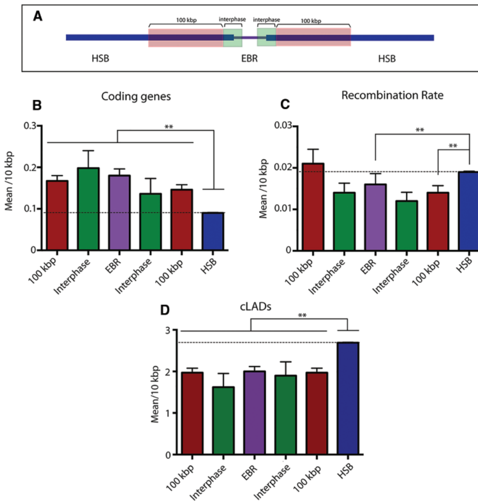
Fig. 3. —Genome wide analysis of gene content and recombination rates. (A) Schematic representation of the genomic regions considered for the analysis (see “Materials and methods” section for details). (B) Distribution of protein-coding genes. The X-axis represents the genomic regions analyzed, whereas the Y-axis displays the mean number of genes detected per 10 kbp. (C) Distribution of recombination rates. The X-axis represents the genomic regions analyzed, whereas the Y-axis displays the mean recombination rate detected per 10 kbp. (D) Distribution of constitutive Lamina Associated Domains (cLADs). The X-axis represents the genomic regions analyzed, whereas the Y-axis displays the mean number of cLADs identified per each 10 kbp windows. Standard error bars are represented. Punctuated lines represent genome-wide means. Asterisk indicates statistical significance (Kruskal–Wallis test, **P -value < 0.001).
