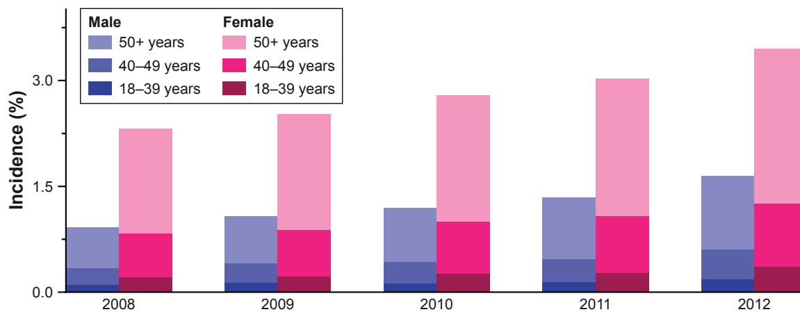
Figure 4 Annual incidence of dry eye disease by sex and age, 2008–2012.
