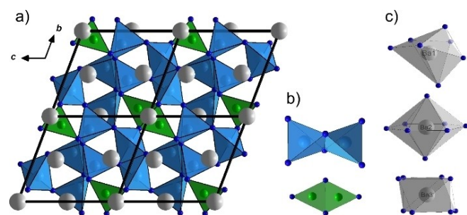
Figure 1. Crystal structure representation of \text{Ba}_2[\text{BeAl}_3\text{N}_5]:\text{Eu}^{2+} with Al atoms (light blue), Be atoms (green), N atoms (blue) and Ba atoms (gray). a) view of 2 \times 2 \times 2 -unit cells along [100]; b) bow-tie unit [\text{Al}_2\text{N}_6]^{12-} (top, light blue) and [\text{Be}_2\text{N}_4]^{8-} unit (bottom, green); c) coordination polyhedra (gray) around Ba1 (top), Ba2 (middle) and Ba3 (bottom).
