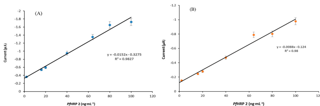
Figure 5. Linear regression analysis of the chronoamperometric response of PfHRP 2 detection in buffer (PBS, 0.01M, pH 7.4, spiked with 1–100 \text{ng}\cdot\text{mL}^{-1} PfHRP 2 ) (A) and 100% serum samples (spiked with 1–100 \text{ng}\cdot\text{mL}^{-1} PfHRP 2 ) (B) on a JD2 sensor. Measurements were conducted at -0.2 \text{ V} . Correlation coefficient and R^2 value of 0.9827 for the buffer matrix and 0.98 for the serum matrix ( n = 3 ).
