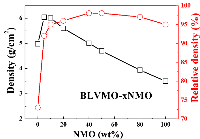
Figure 1. Bulk and relative densities of (100− x ) wt.% (Bi 0.95 Li 0.05 )(V 0.9 Mo 0.1 )O 4 (BLVMO)− x wt.% Na 2 Mo 2 O 7 (NMO) ceramic composites.
