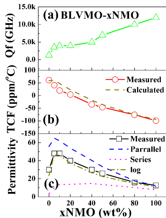
Figure 5. The microwave properties of (100-x) wt.% BLVMO- x wt.% NMO ceramic composites as a function of x (NMO fraction). (a) Q_f , (b) TCF, (c) \epsilon_r .
