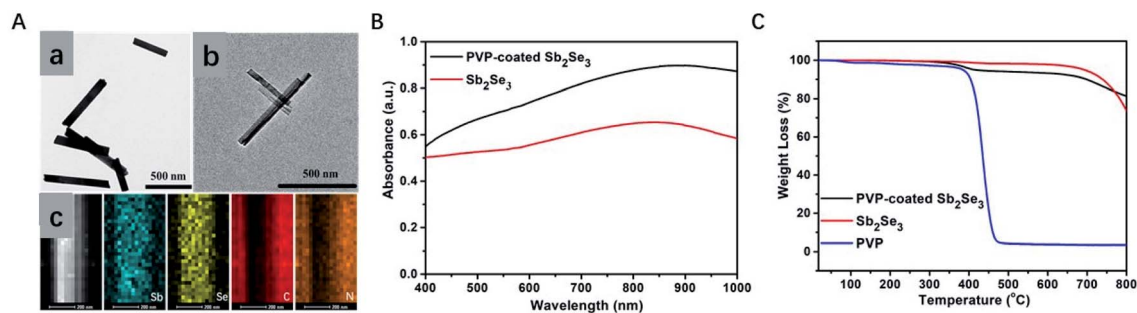
Fig. 1 TEM images of \text{Sb}_2\text{Se}_3 (A-a) and PVP-coated \text{Sb}_2\text{Se}_3 nanorods (A-b) and (A-c) EDX elemental mapping images of PVP-coated \text{Sb}_2\text{Se}_3 nanorods. (B) UV-vis-NIR absorption spectra of \text{Sb}_2\text{Se}_3 and PVP-coated \text{Sb}_2\text{Se}_3 nanorods aqueous solution. (C) TGA curves of PVP, \text{Sb}_2\text{Se}_3 and PVP-coated \text{Sb}_2\text{Se}_3 nanorods.
