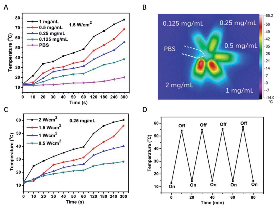
Fig. 2 (A) Temperature changes of PVP-coated \text{Sb}_2\text{Se}_3 nanorods at different concentrations exposed to 808 nm laser at a power density of 1.5 \text{ W cm}^{-2} . (B) Infrared thermal images of the solution containing PVP-coated \text{Sb}_2\text{Se}_3 nanorods under the NIR laser ( 808 \text{ nm} , 1.0 \text{ W cm}^{-2} ) irradiation for 5 min. (C) Temperature change of PVP-coated \text{Sb}_2\text{Se}_3 nanorods at a constant concentration with different power. (D) Temperature variation of PVP-coated \text{Sb}_2\text{Se}_3 nanorods aqueous solution under 808 nm laser irradiation ( 1.0 \text{ W cm}^{-2} ) for four laser on/off cycles.
