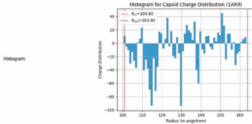
Figure 4. Physical properties analysis. Histogram showing the charge distribution of a selected capsid PDB ID, where R_{in} represents inner capsid radii and R_{out} represents outer capsid radii.
