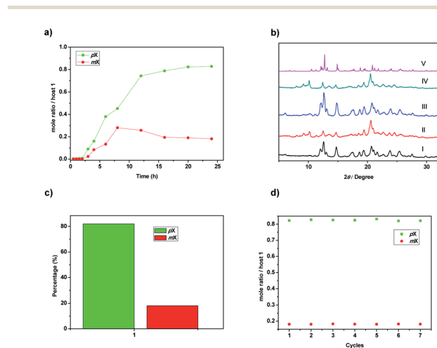
Fig. 4 (a) Time-dependent solid–vapor sorption plot of activated 1 for pX and mX equimolar mixture vapor. (b) PXRD patterns of 1 : (I) activated 1 adsorption of pX vapour for 20 h; (II) activated 1 adsorption of mX vapour for 20 h; (III) activated 1 adsorption of pX/mX mixture vapour for 20 h; (IV) activated 1 after adsorption of pX/mX mixture vapour for 20 h and then heating at 150 °C under vacuum for 3 h; (V) simulated from single-crystal structure of 1@pX . (c) Relative uptakes of pX and mX adsorbed by activated 1 that adsorbed pX/mX mixtures for 20 h as measured by gas chromatography. (d) Relative uptakes of pX and mX by activated 1 that adsorbed pX/mX mixtures for 20 h after seven recycles.
