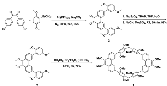
Scheme 1 Synthesis of host 1 .
