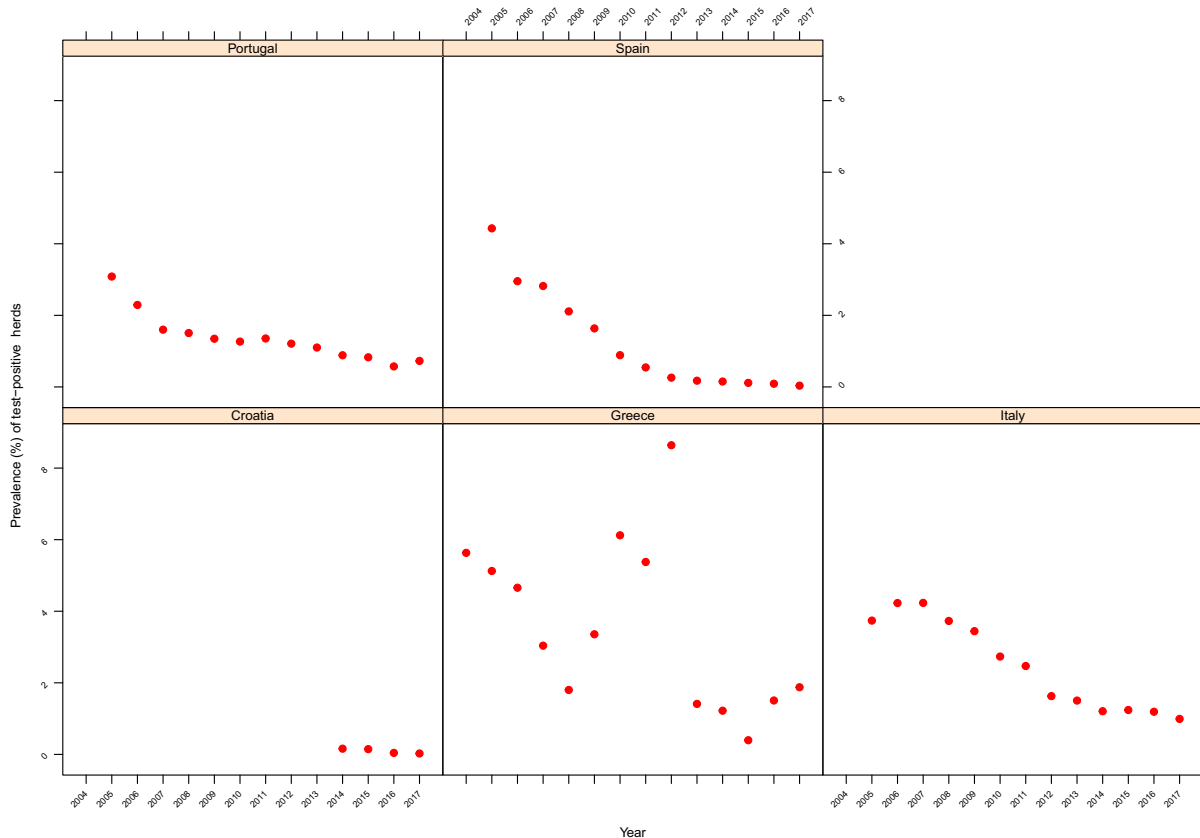
Figure 49: Prevalence of Brucella melitensis test-positive sheep and goat herds, in Croatia, Greece, Italy, Portugal and Spain, 2004–2017
