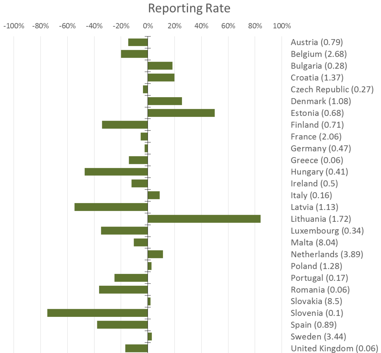
Figure 68: Food-borne (including waterborne) outbreaks reporting rate (per 100,000 population) in 2017 (in brackets), by EU Member State and % of difference compared with 2016 (green bars)
