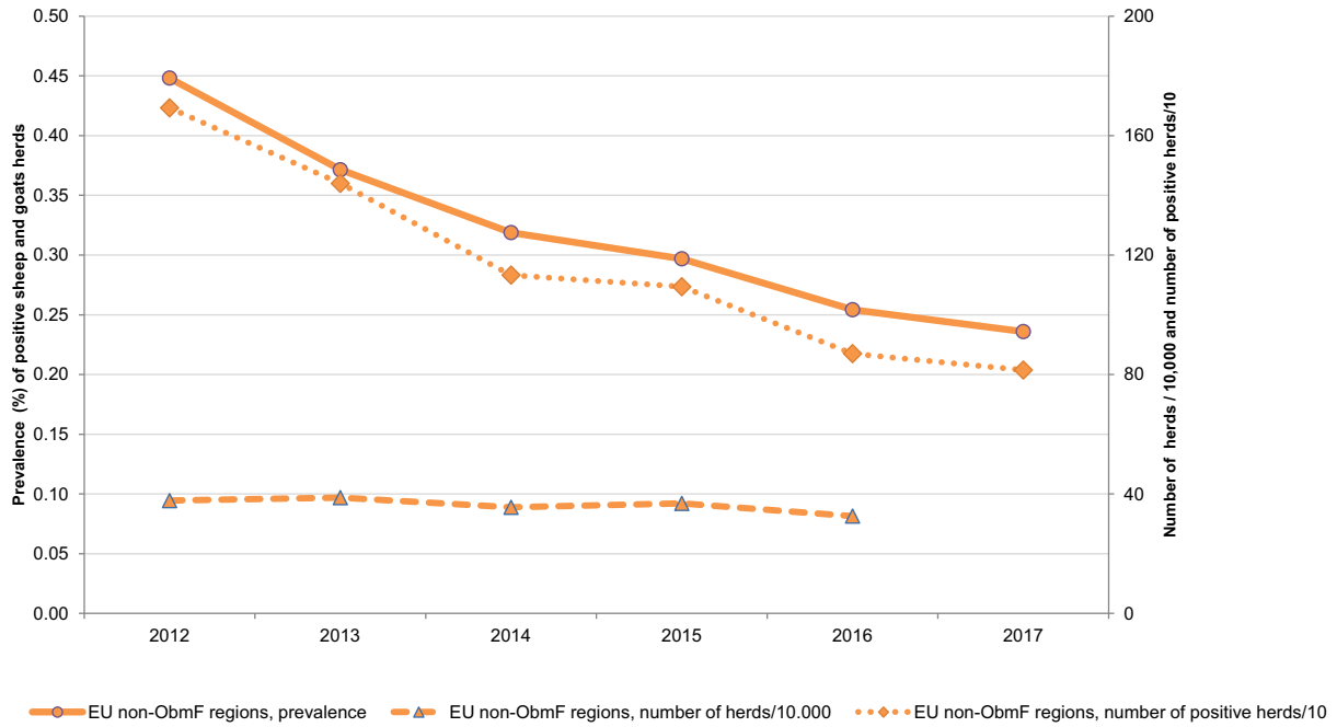
Figure 48: Proportion of sheep flocks and goat herds infected with or positive for B. melitensis , in non-ObmF regions, EU, 2012–2017
