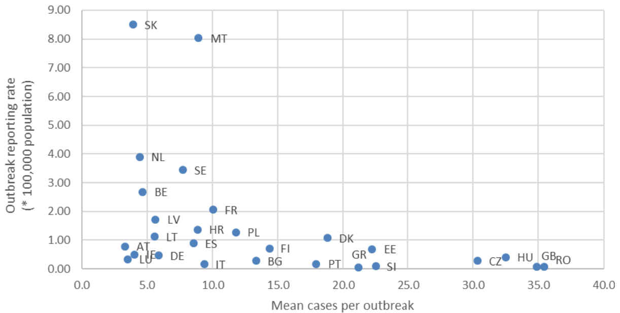
Figure 69: Mean number of human cases per outbreak (food-borne including waterborne outbreaks) and outbreak reporting rate (per 100,000 population), by reporting Member State, EU, 2017
