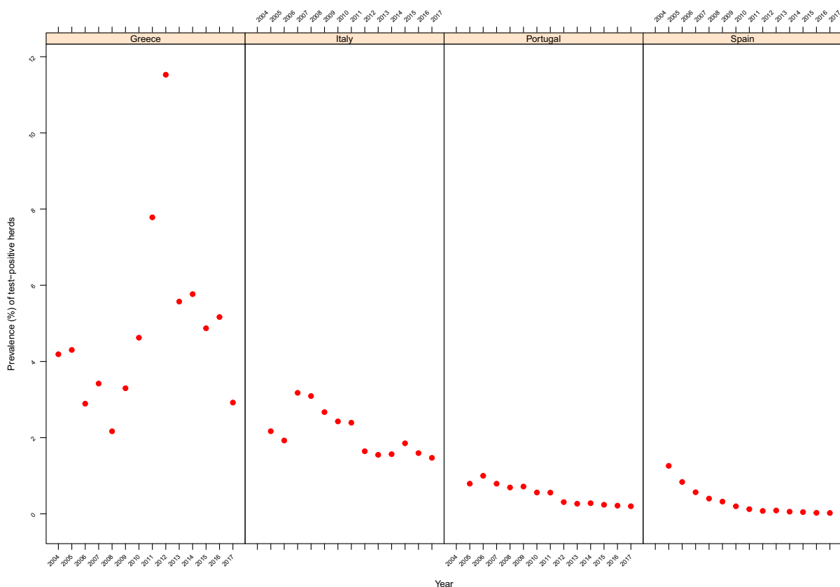
Figure 46: Prevalence of Brucella test-positive cattle herds, in Greece, Italy, Portugal and Spain, 2004–2017
