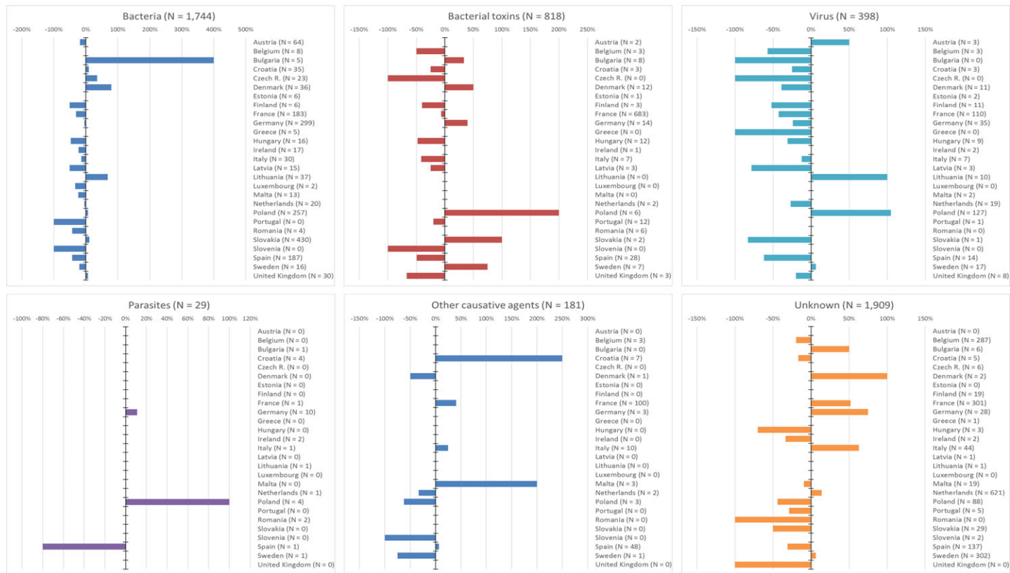
Figure 70: Food-borne (including waterborne outbreaks) reported in EU in 2017, by reporting Member States and by type of pathogen and % of difference compared with 2016
