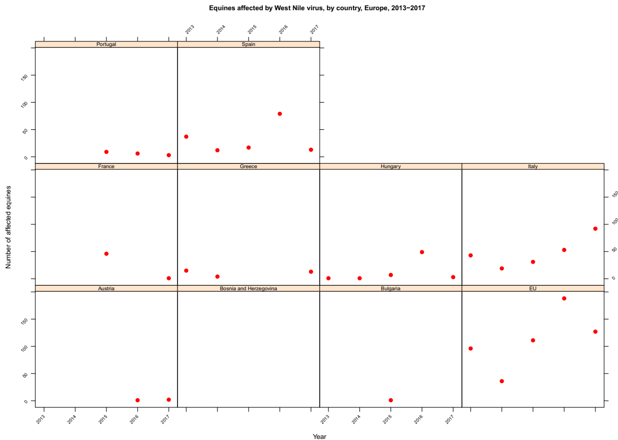
Figure 62: Number of affected equines reported to the EU Animal Disease Notification System (ADNS), by reporting MS, EU, 2013–2017
