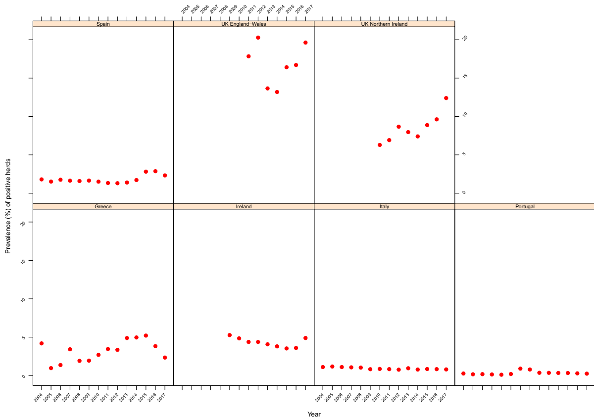
Figure 41: Prevalence of bovine tuberculosis test-positive cattle herds, in non-OTF regions of five non-OTF cofinanced Member States and of one non-OTF not funded Member State Greece, 2004–2017
