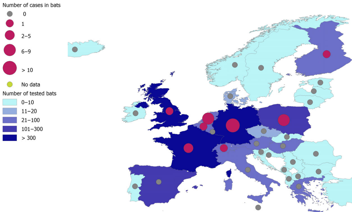
Figure 59: The geographical distribution of reported rabies cases (EBLV-1 or EBLV-2 or other species) in bats and the number of tested bats, by reporting country, EU, 2017
