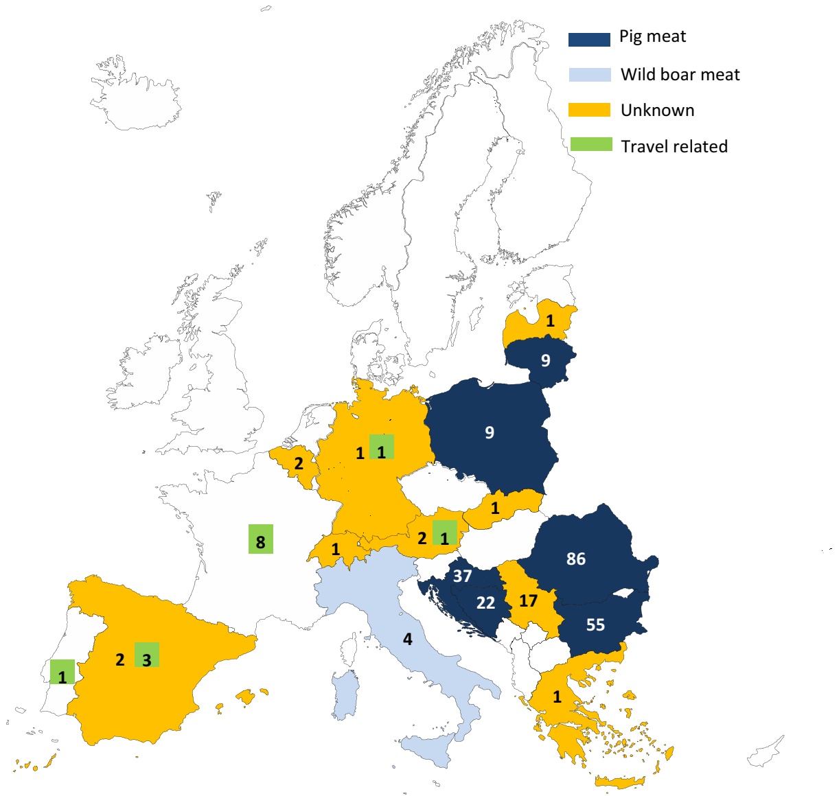
Countries in which human cases were reported due to food-borne outbreaks (EFSA data) are in colour according the food vehicle causing the outbreaks ('pigmeat', 'wild-boar meat' or 'unknown' food vehicle). The number of cases in each country indicates domestic trichinellosis cases (ECDC data); numbers in green box indicate the travel-related trichinellosis human cases.
