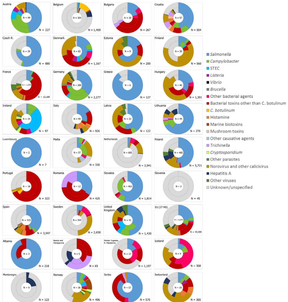
Figure 72: Frequency distribution of food-borne (including waterborne) outbreaks (internal circle) and human cases involved in outbreaks (external circle), by reporting EU Member States and non-Member States (bottom figure), by causative agent, 2017
