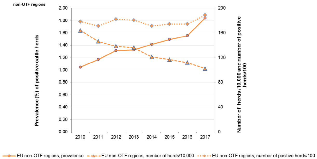
Figure 40: Proportion of cattle herds positive for bovine tuberculosis in non-OTF regions, EU, 2010–2017
