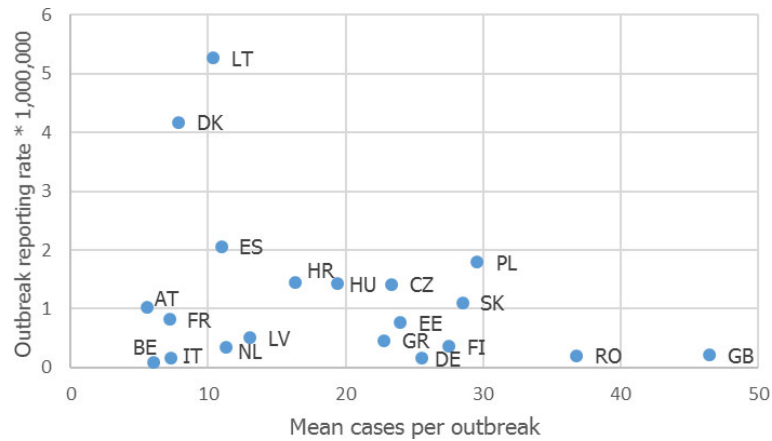
Figure 74: Mean number of cases per outbreak and reporting rate of general food-borne (including waterborne) outbreaks of salmonellosis (per million population) reported in the EU, by reporting Member State, 2017
