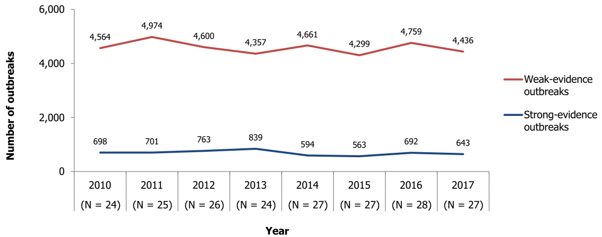
Figure 67: Number of food-borne (including waterborne) outbreaks in the reporting Member States, EU, 2010–2017
