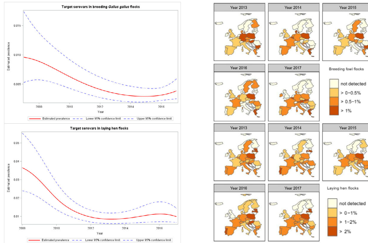
Figure 17: Estimate of the trend prevalence of poultry flocks positive for target Salmonella serovars, at the EU level, in different poultry animal populations, EU, 2007–2017
