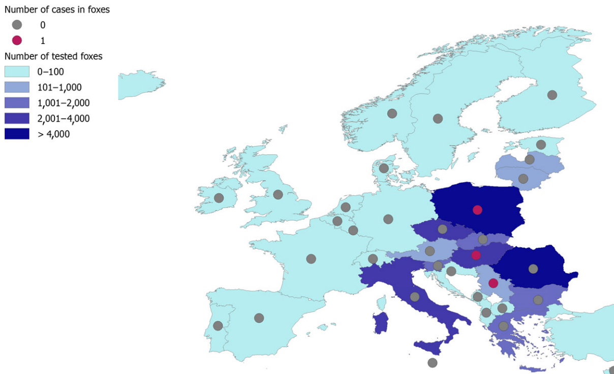
Figure 58: The geographical distribution of the reported rabies cases in foxes and the number of tested foxes, by reporting country, EU, 2017
