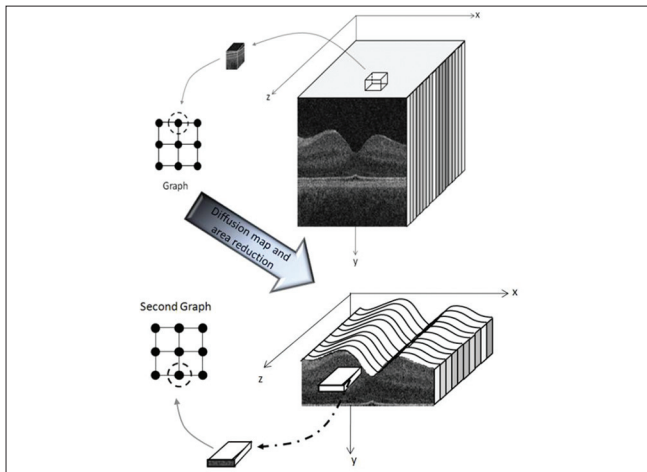
Figure 17: Construction of graph nodes from a 3D OCT [42]
