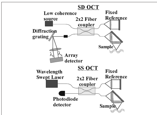
Figure 3: Fourier domain configurations. Spectral domain OCT utilizes a spectrometer in the detection arm, whereas swept source OCT requires a wavelength swept laser and a standard photodiode detector
