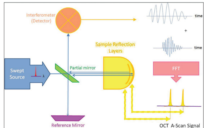
Figure 1: Block-diagram of optical coherence tomography
