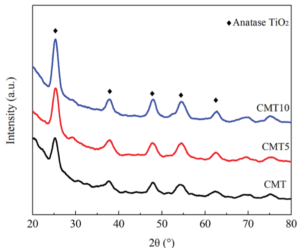
Fig. 5 XRD patterns of the catalyst samples.
