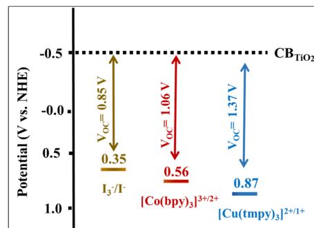
Fig. 14 Redox potential values and the corresponding V_{\text{OC}} values of the most common and efficient redox couples used in DSSCs, including \text{I}_3^-/\text{I}^- , [\text{Co}(\text{bpy})_3]^{3+}/^{2+} , and [\text{Cu}(\text{tmpy})_3]^{2+}/^{1+} .
