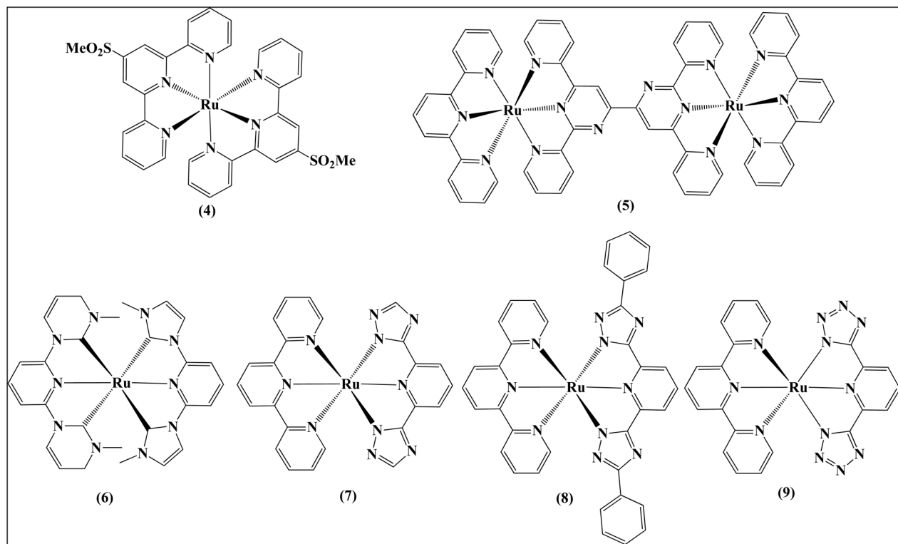
Fig. 8 Tridentate heteroleptic Ru(III) complexes (4–9).
