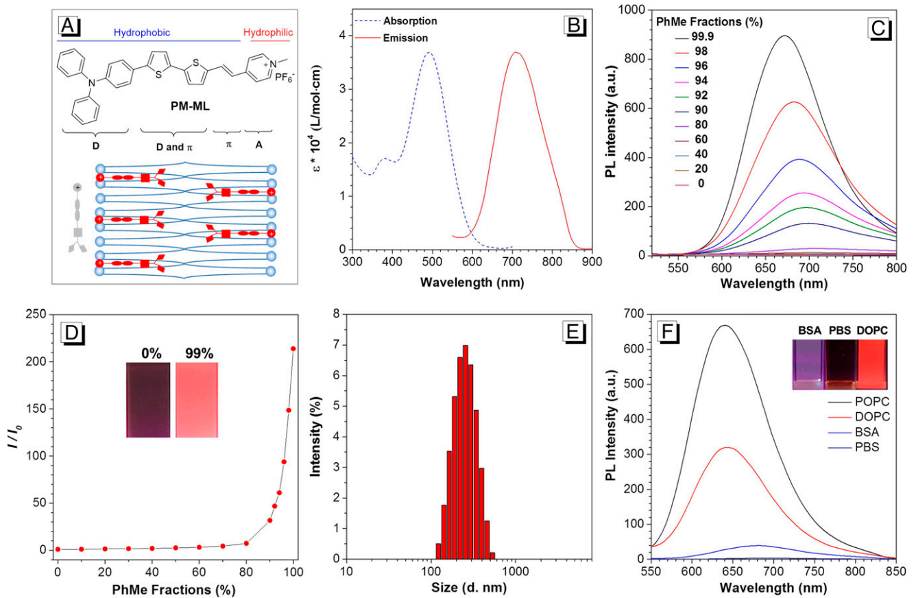
Fig. 1. Structure and photophysical properties of PM-ML. (A) The chemical structure, schematic illustration of PM-ML structural characteristics, and its interaction with membrane structure. (B) The molar absorption coefficient of PM-ML in DMSO and its emission spectrum in the solid state. (C) Photoluminescence (PL) spectra of PM-ML (10 \mu M) in the mixtures of DMSO and toluene (PhMe) with different PhMe fractions. (D) The plot of the relative emission intensity of PM-ML versus PhMe fractions. I_0 and I are the peak values of PL intensities of PM-ML in DMSO and DMSO/PhMe mixtures, respectively. (Inset) Fluorescence images of PM-ML in DMSO solution (0% PhMe) and aggregated state (99% PhMe) with 365-nm excitation. (E) Size distribution of PM-ML in the mixture of DMSO/PhMe with 99% PhMe content measured by dynamic light scattering. (F) PL spectra of PM-ML (10 \mu M) in phosphate-buffered saline (PBS) solution with 3 mg \cdot mL -1 phospholipids (POPC or DOPC) or proteins (BSA). (Inset) Corresponding fluorescence images of PM-ML in PBS solution, DOPC, or BSA under a hand-held ultraviolet lamp at 365 nm.
